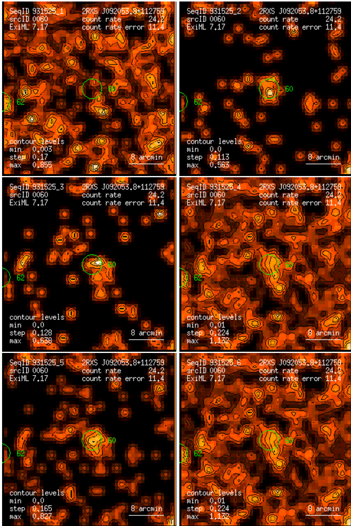
Figure 60: RASS 931525: detection 0060: band rate images, Gaussian filter: (1) PSPC channels 11 – 41, (2) 52 – 90, (3) 91 – 201, (4) 11 – 235, (5) 52 – 201, (6) 11 – 201. Broad band rates in counts/ks. Band rate contour levels in counts/ks/arcmin 2 .
