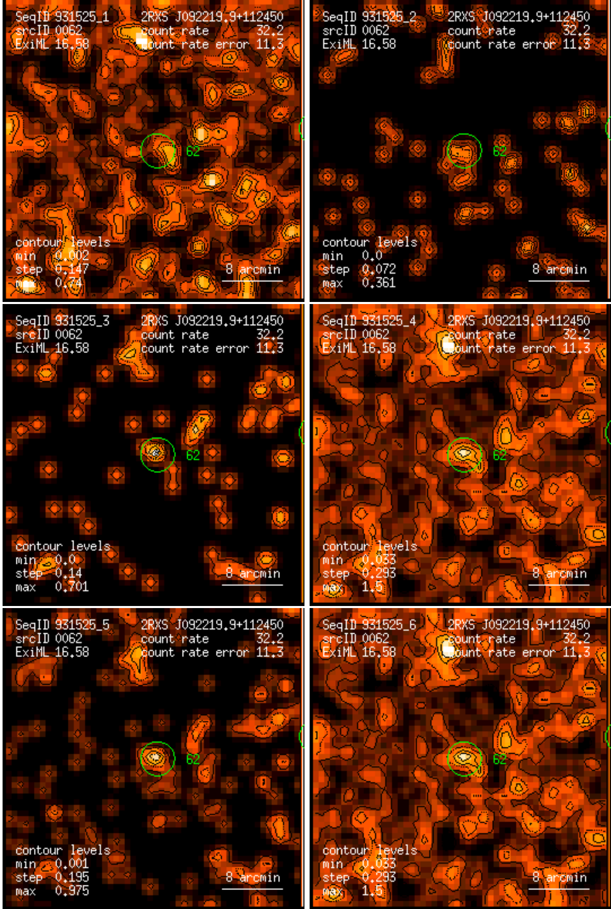
Figure 62: RASS 931525: detection 0062: band rate images, Gaussian filter: (1) PSPC channels 11 – 41, (2) 52 – 90, (3) 91 – 201, (4) 11 – 235, (5) 52 – 201, (6) 11 – 201. Broad band rates in counts/ks. Band rate contour levels in counts/ks/arcmin 2 .
