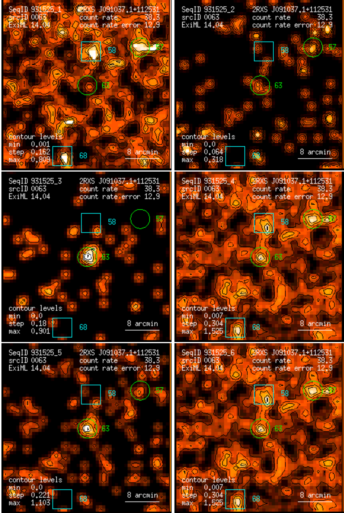
Figure 63: RASS 931525: detection 0063: band rate images, Gaussian filter: (1) PSPC channels 11 – 41, (2) 52 – 90, (3) 91 – 201, (4) 11 – 235, (5) 52 – 201, (6) 11 – 201. Broad band rates in counts/ks. Band rate contour levels in counts/ks/arcmin 2 .
