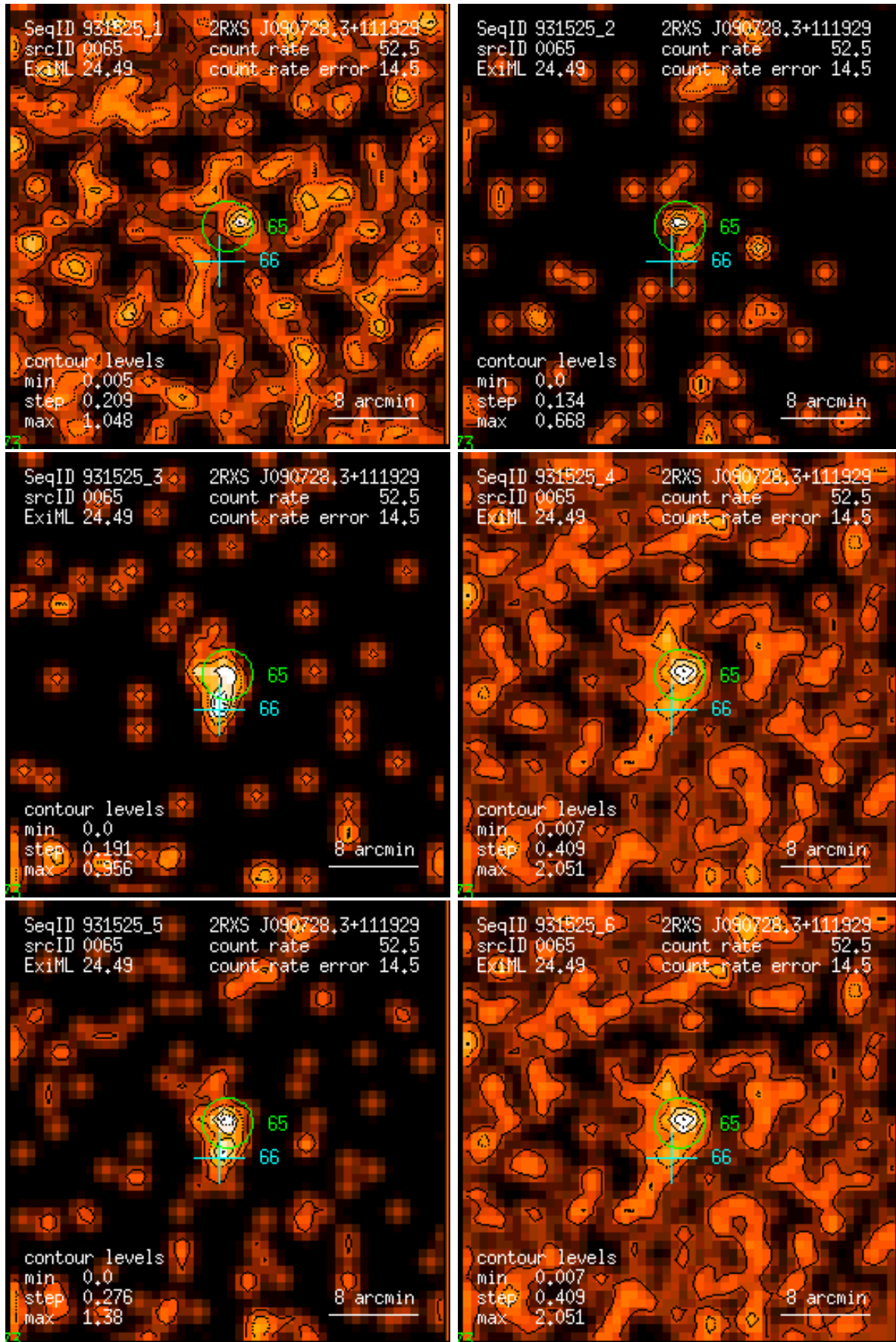
Figure 65: RASS 931525: detection 0065: band rate images, Gaussian filter: (1) PSPC channels 11 – 41, (2) 52 – 90, (3) 91 – 201, (4) 11 – 235, (5) 52 – 201, (6) 11 – 201. Broad band rates in counts/ks. Band rate contour levels in counts/ks/arcmin 2 .
