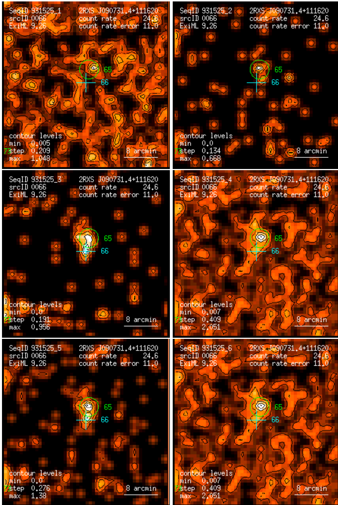
Figure 66: RASS 931525: detection 0066: band rate images, Gaussian filter: (1) PSPC channels 11 – 41, (2) 52 – 90, (3) 91 – 201, (4) 11 – 235, (5) 52 – 201, (6) 11 – 201. Broad band rates in counts/ks. Band rate contour levels in counts/ks/arcmin 2 .
