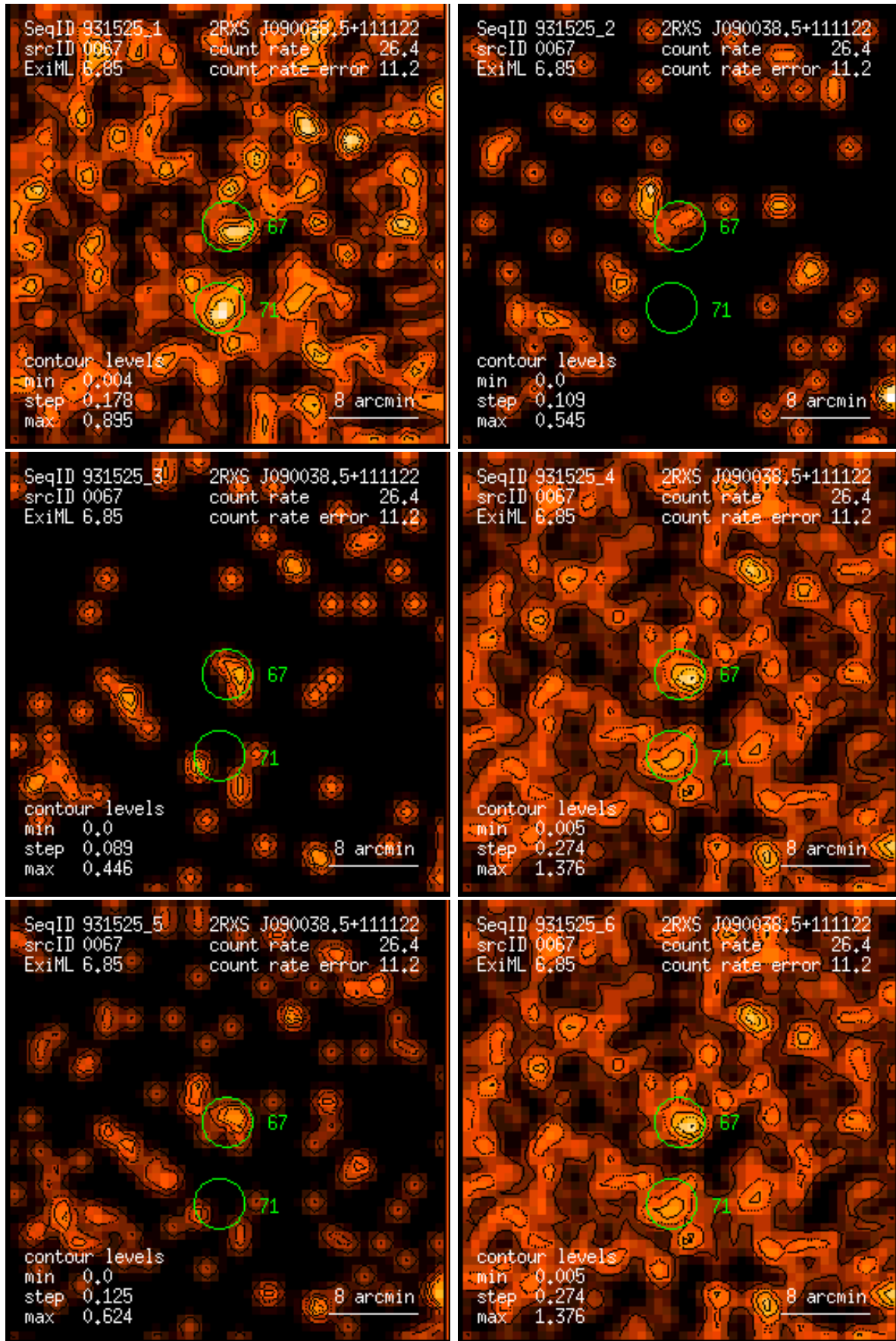
Figure 67: RASS 931525: detection 0067: band rate images, Gaussian filter: (1) PSPC channels 11 – 41, (2) 52 – 90, (3) 91 – 201, (4) 11 – 235, (5) 52 – 201, (6) 11 – 201. Broad band rates in counts/ks. Band rate contour levels in counts/ks/arcmin 2 .
