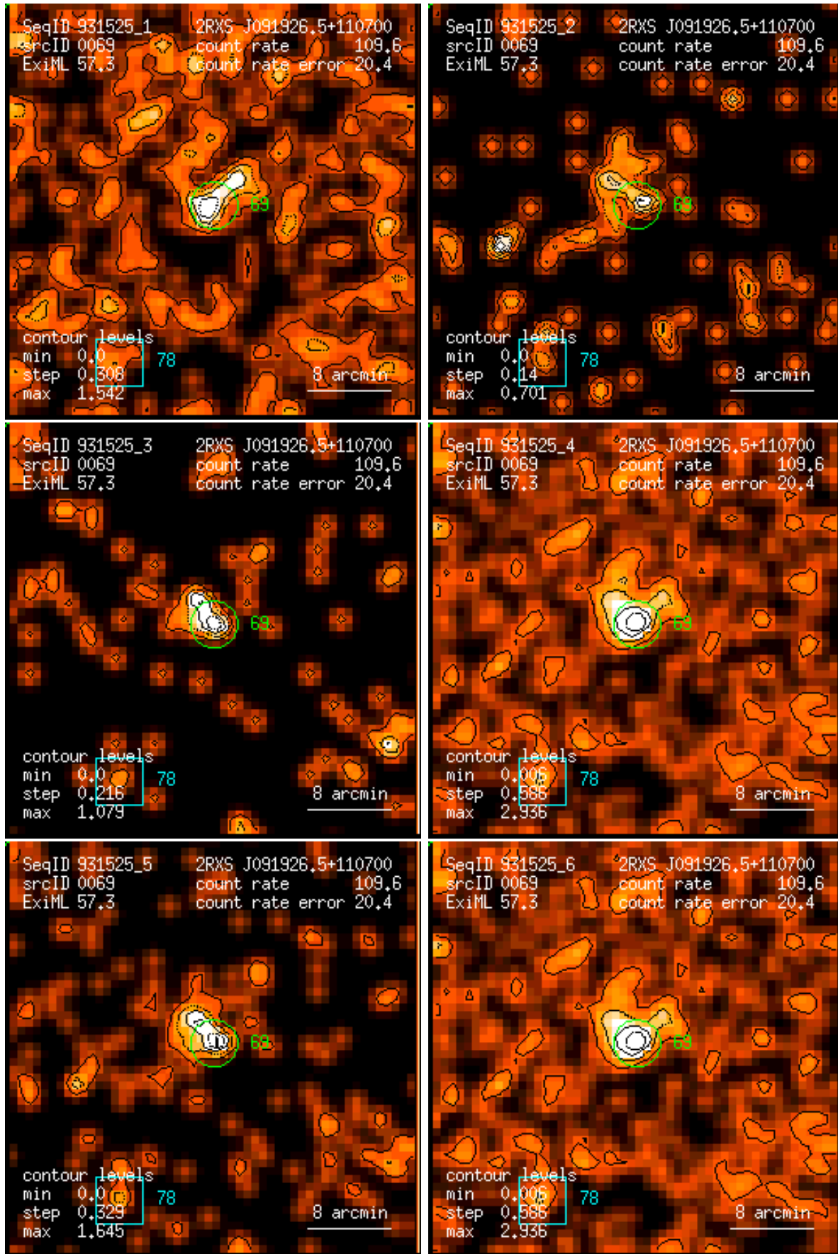
Figure 69: RASS 931525: detection 0069: band rate images, Gaussian filter: (1) PSPC channels 11 – 41, (2) 52 – 90, (3) 91 – 201, (4) 11 – 235, (5) 52 – 201, (6) 11 – 201. Broad band rates in counts/ks. Band rate contour levels in counts/ks/arcmin 2 .
