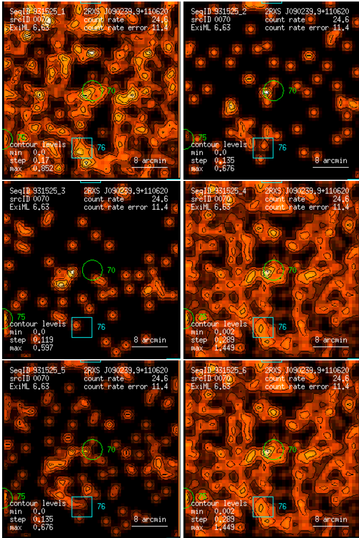
Figure 70: RASS 931525: detection 0070: band rate images, Gaussian filter: (1) PSPC channels 11 – 41, (2) 52 – 90, (3) 91 – 201, (4) 11 – 235, (5) 52 – 201, (6) 11 – 201. Broad band rates in counts/ks. Band rate contour levels in counts/ks/arcmin 2 .
