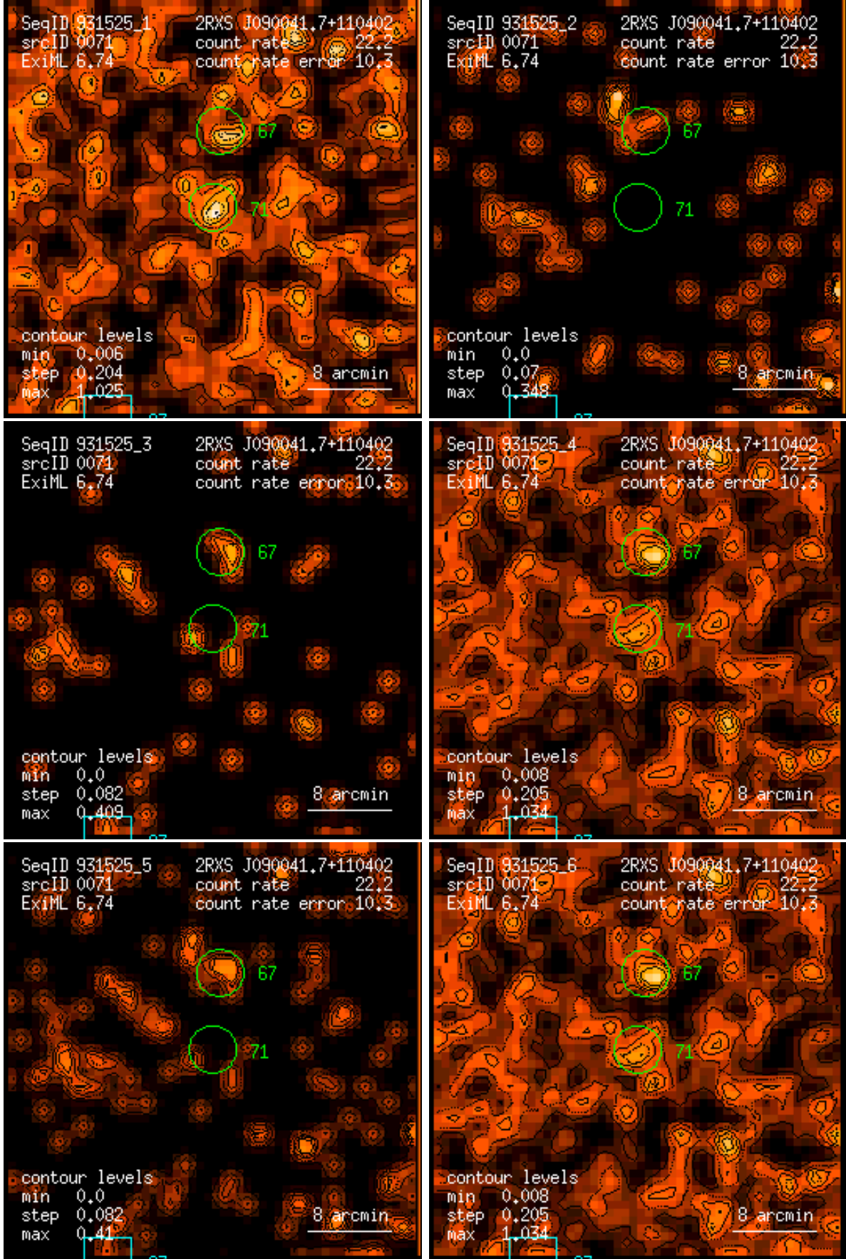
Figure 71: RASS 931525: detection 0071: band rate images, Gaussian filter: (1) PSPC channels 11 – 41, (2) 52 – 90, (3) 91 – 201, (4) 11 – 235, (5) 52 – 201, (6) 11 – 201. Broad band rates in counts/ks. Band rate contour levels in counts/ks/arcmin 2 .
