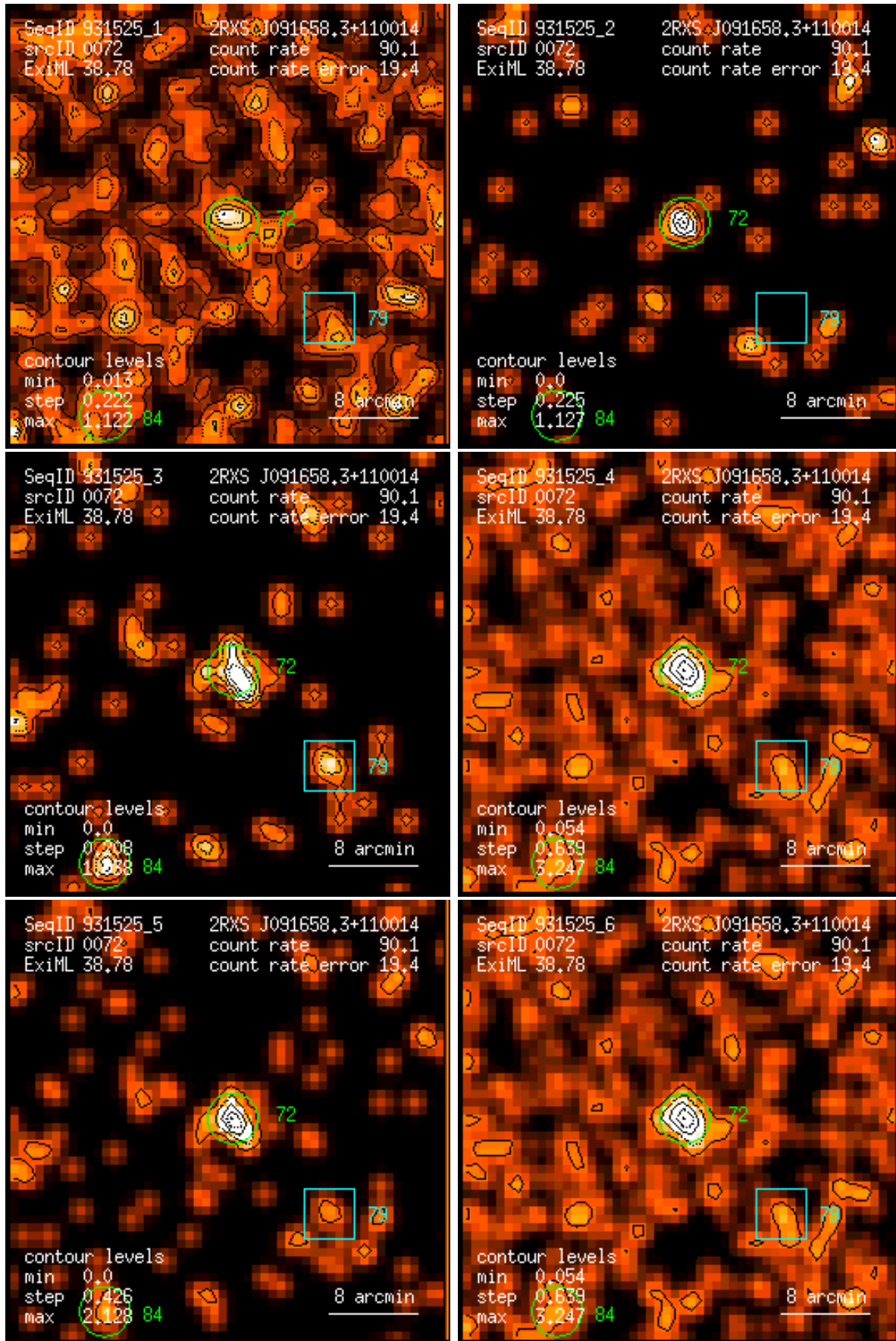
Figure 72: RASS 931525: detection 0072: band rate images, Gaussian filter: (1) PSPC channels 11 – 41, (2) 52 – 90, (3) 91 – 201, (4) 11 – 235, (5) 52 – 201, (6) 11 – 201. Broad band rates in counts/ks. Band rate contour levels in counts/ks/arcmin 2 .
