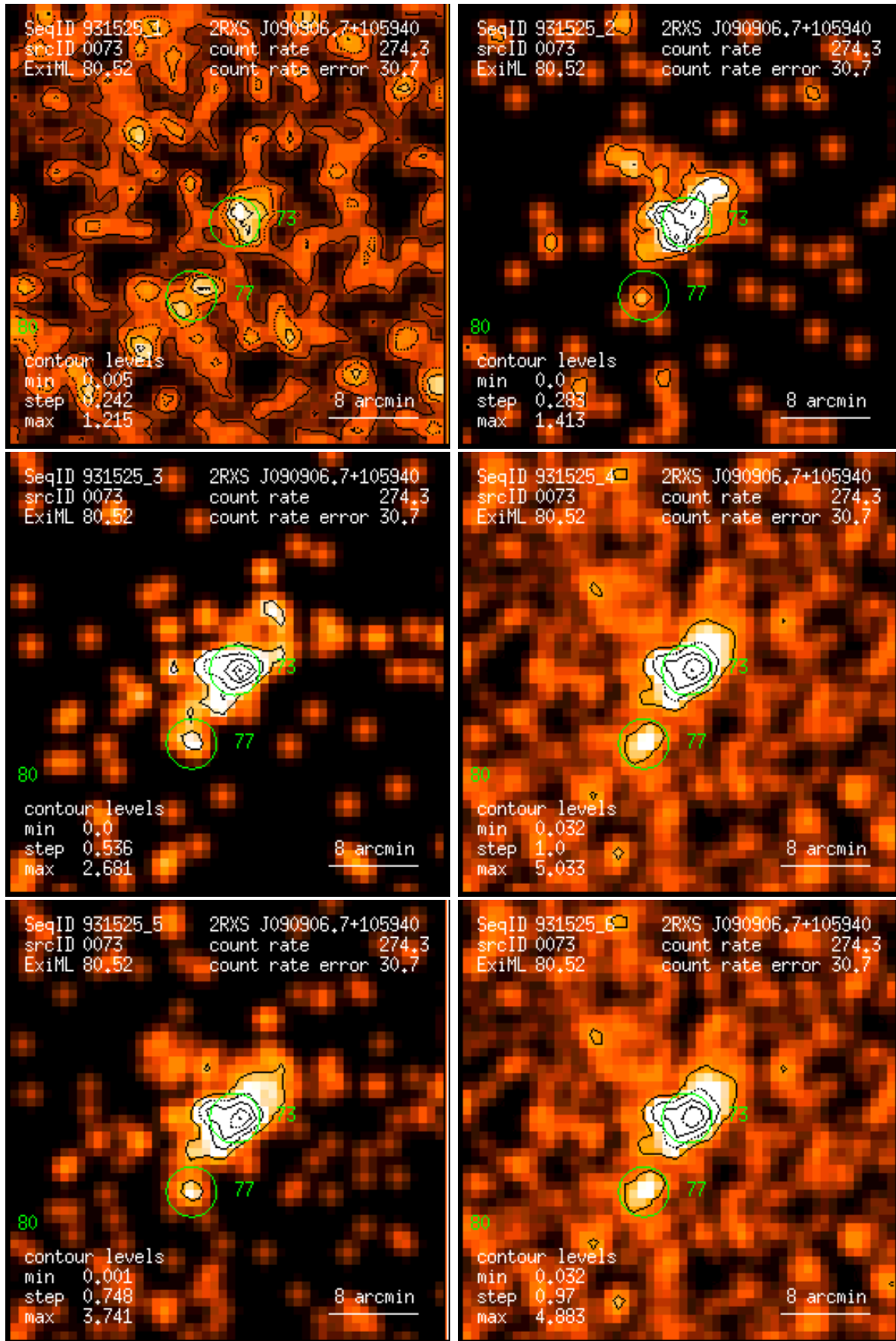
Figure 73: RASS 931525: detection 0073: band rate images, Gaussian filter: (1) PSPC channels 11 – 41, (2) 52 – 90, (3) 91 – 201, (4) 11 – 235, (5) 52 – 201, (6) 11 – 201. Broad band rates in counts/ks. Band rate contour levels in counts/ks/arcmin 2 .
