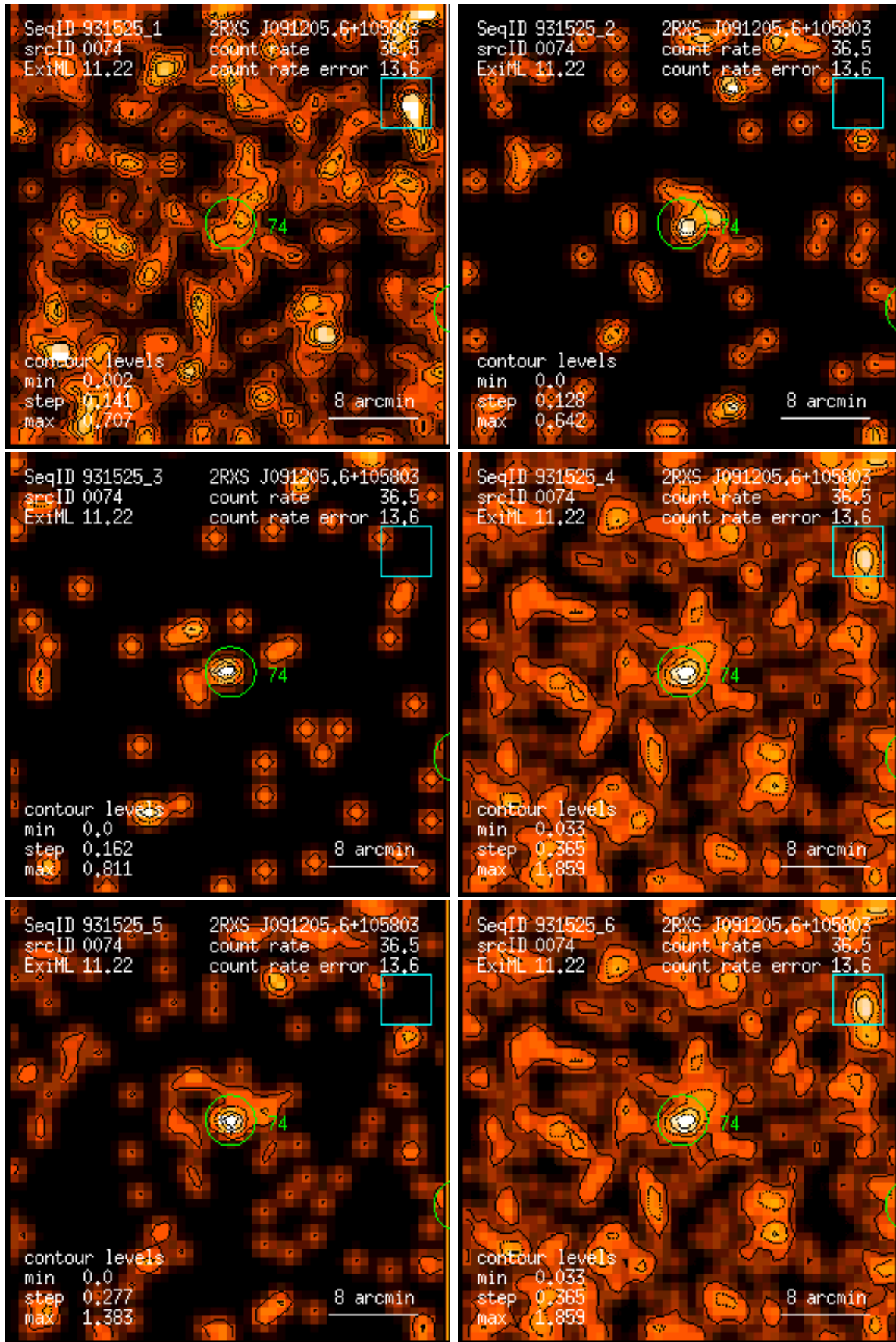
Figure 74: RASS 931525: detection 0074: band rate images, Gaussian filter: (1) PSPC channels 11 – 41, (2) 52 – 90, (3) 91 – 201, (4) 11 – 235, (5) 52 – 201, (6) 11 – 201. Broad band rates in counts/ks. Band rate contour levels in counts/ks/arcmin 2 .
