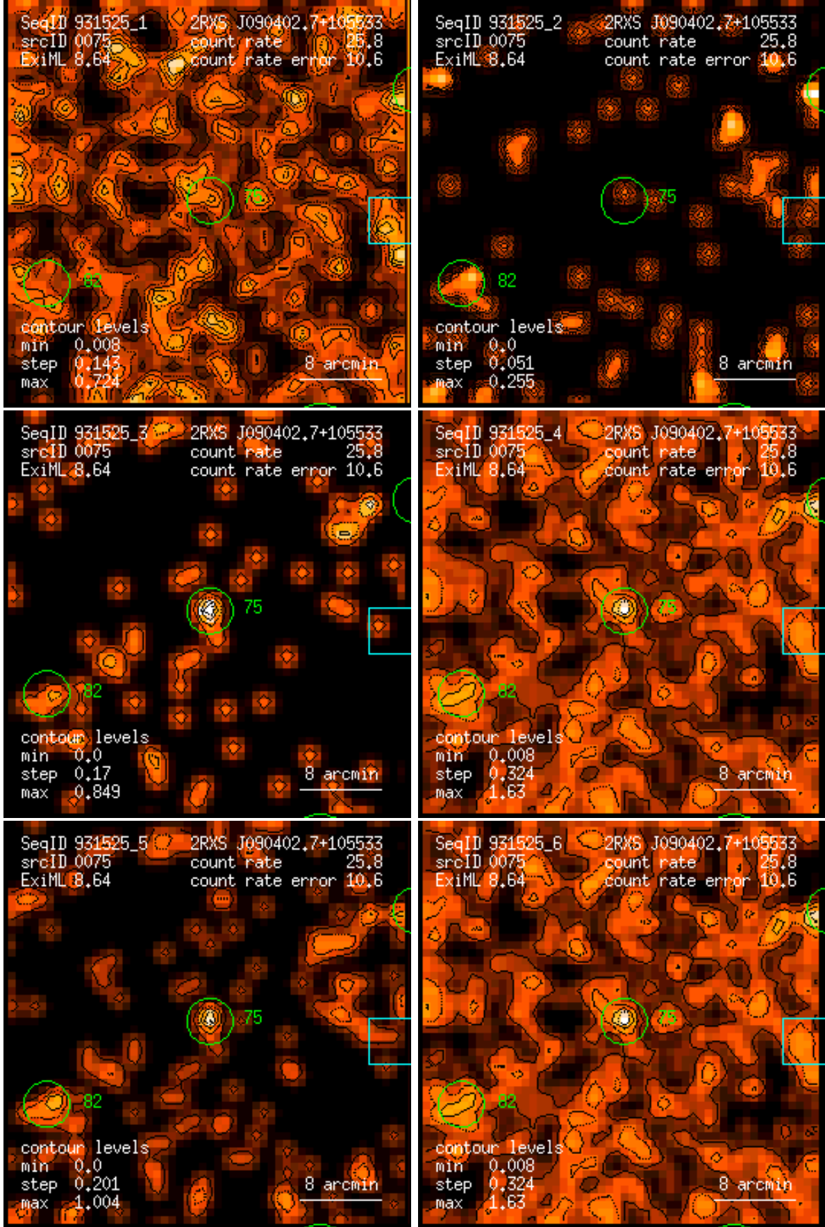
Figure 75: RASS 931525: detection 0075: band rate images, Gaussian filter: (1) PSPC channels 11 – 41, (2) 52 – 90, (3) 91 – 201, (4) 11 – 235, (5) 52 – 201, (6) 11 – 201. Broad band rates in counts/ks. Band rate contour levels in counts/ks/arcmin 2 .
