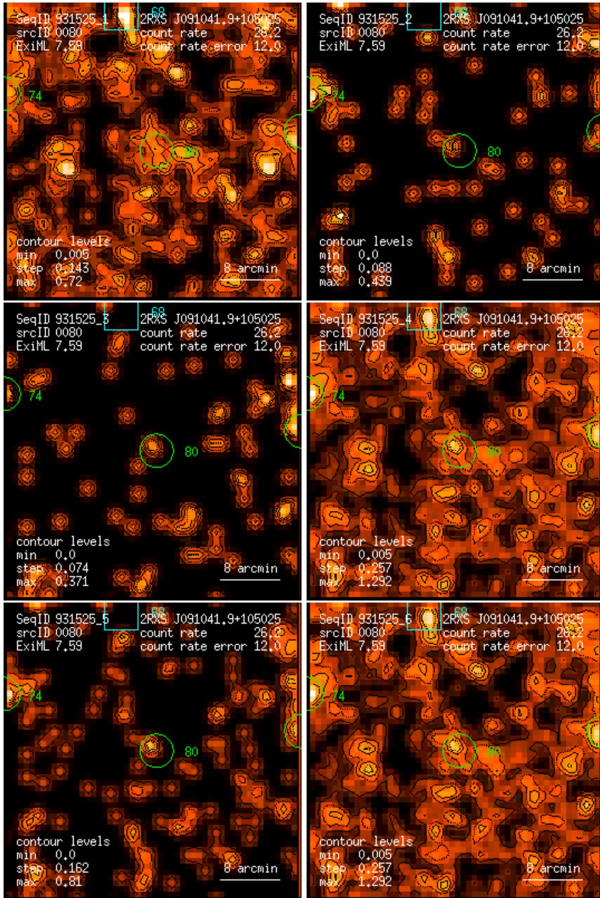
Figure 80: RASS 931525: detection 0080: band rate images, Gaussian filter: (1) PSPC channels 11 – 41, (2) 52 – 90, (3) 91 – 201, (4) 11 – 235, (5) 52 – 201, (6) 11 – 201. Broad band rates in counts/ks. Band rate contour levels in counts/ks/arcmin 2 .
