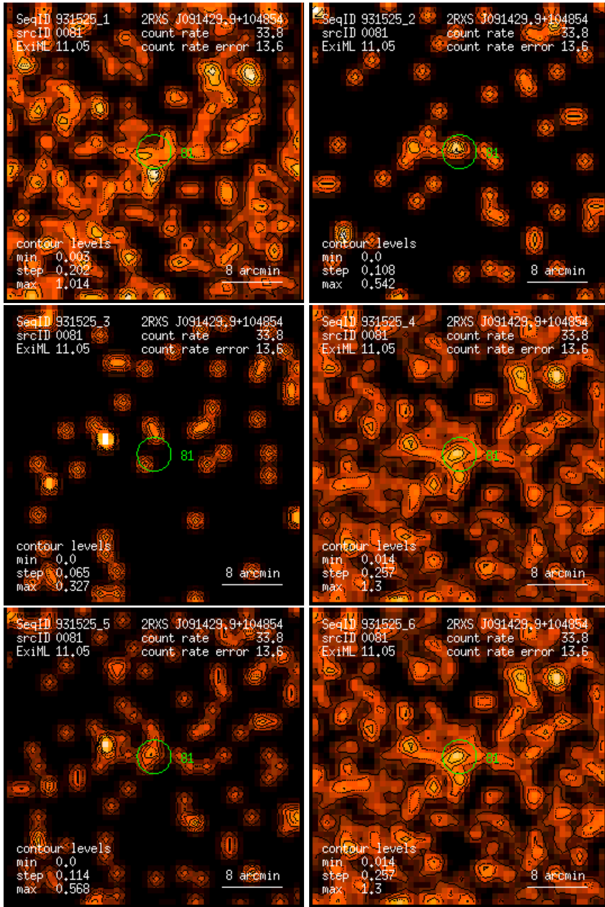
Figure 81: RASS 931525: detection 0081: band rate images, Gaussian filter: (1) PSPC channels 11 – 41, (2) 52 – 90, (3) 91 – 201, (4) 11 – 235, (5) 52 – 201, (6) 11 – 201. Broad band rates in counts/ks. Band rate contour levels in counts/ks/arcmin 2 .
