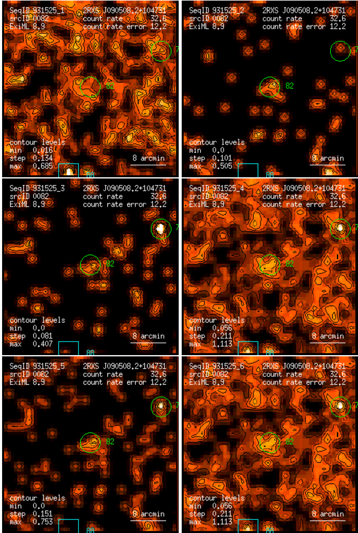
Figure 82: RASS 931525: detection 0082: band rate images, Gaussian filter: (1) PSPC channels 11 – 41, (2) 52 – 90, (3) 91 – 201, (4) 11 – 235, (5) 52 – 201, (6) 11 – 201. Broad band rates in counts/ks. Band rate contour levels in counts/ks/arcmin 2 .
