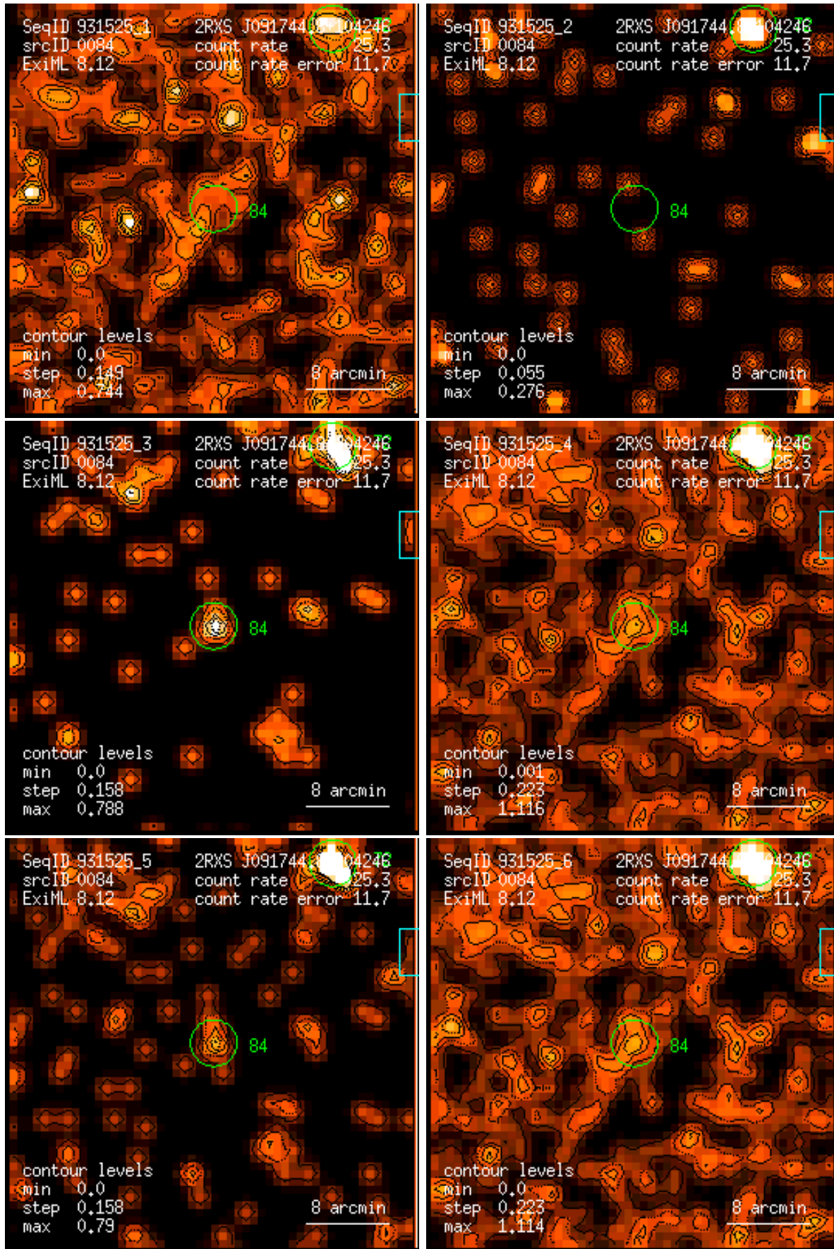
Figure 84: RASS 931525: detection 0084: band rate images, Gaussian filter: (1) PSPC channels 11 – 41, (2) 52 – 90, (3) 91 – 201, (4) 11 – 235, (5) 52 – 201, (6) 11 – 201. Broad band rates in counts/ks. Band rate contour levels in counts/ks/arcmin 2 .
