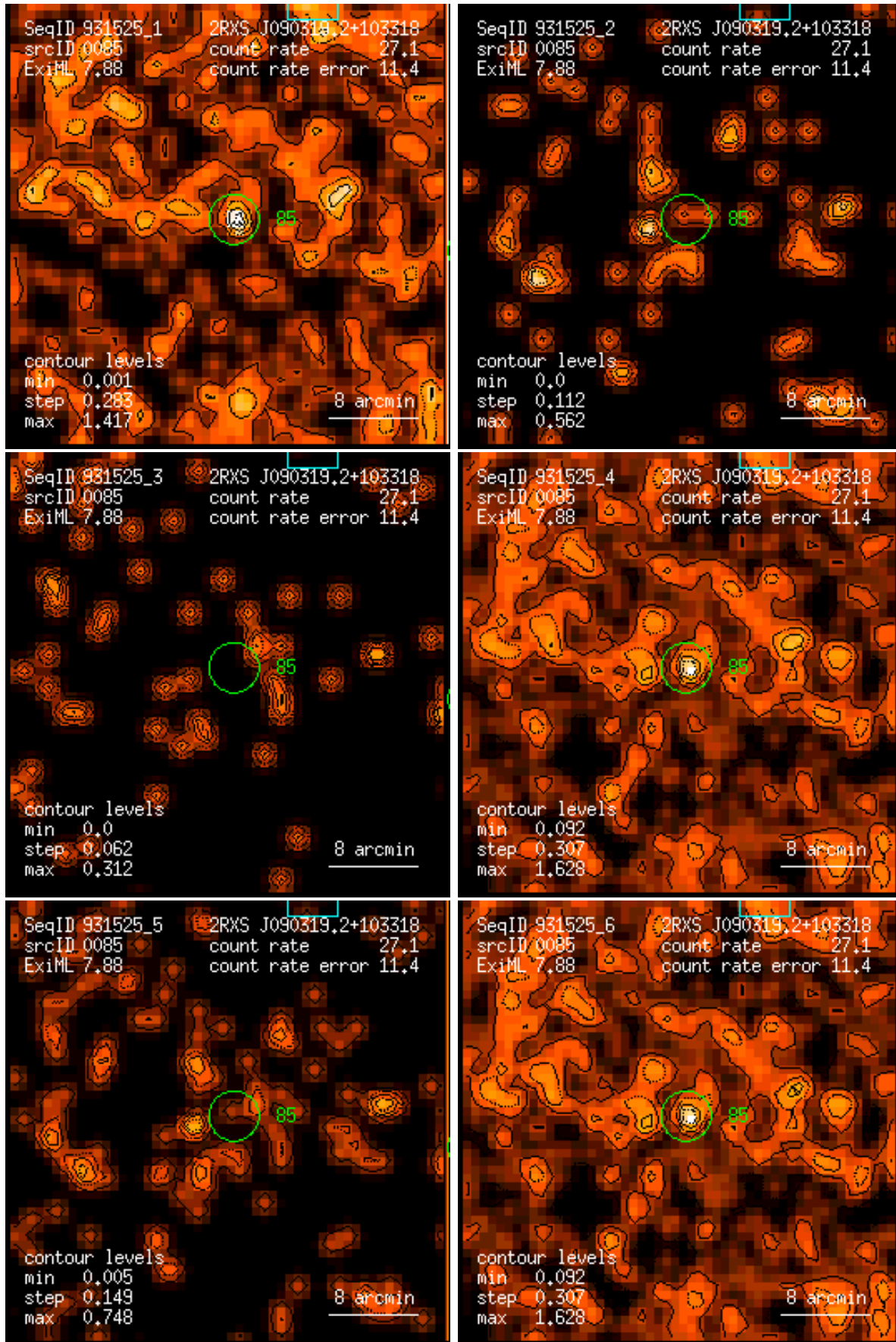
Figure 85: RASS 931525: detection 0085: band rate images, Gaussian filter: (1) PSPC channels 11 – 41, (2) 52 – 90, (3) 91 – 201, (4) 11 – 235, (5) 52 – 201, (6) 11 – 201. Broad band rates in counts/ks. Band rate contour levels in counts/ks/arcmin 2 .
