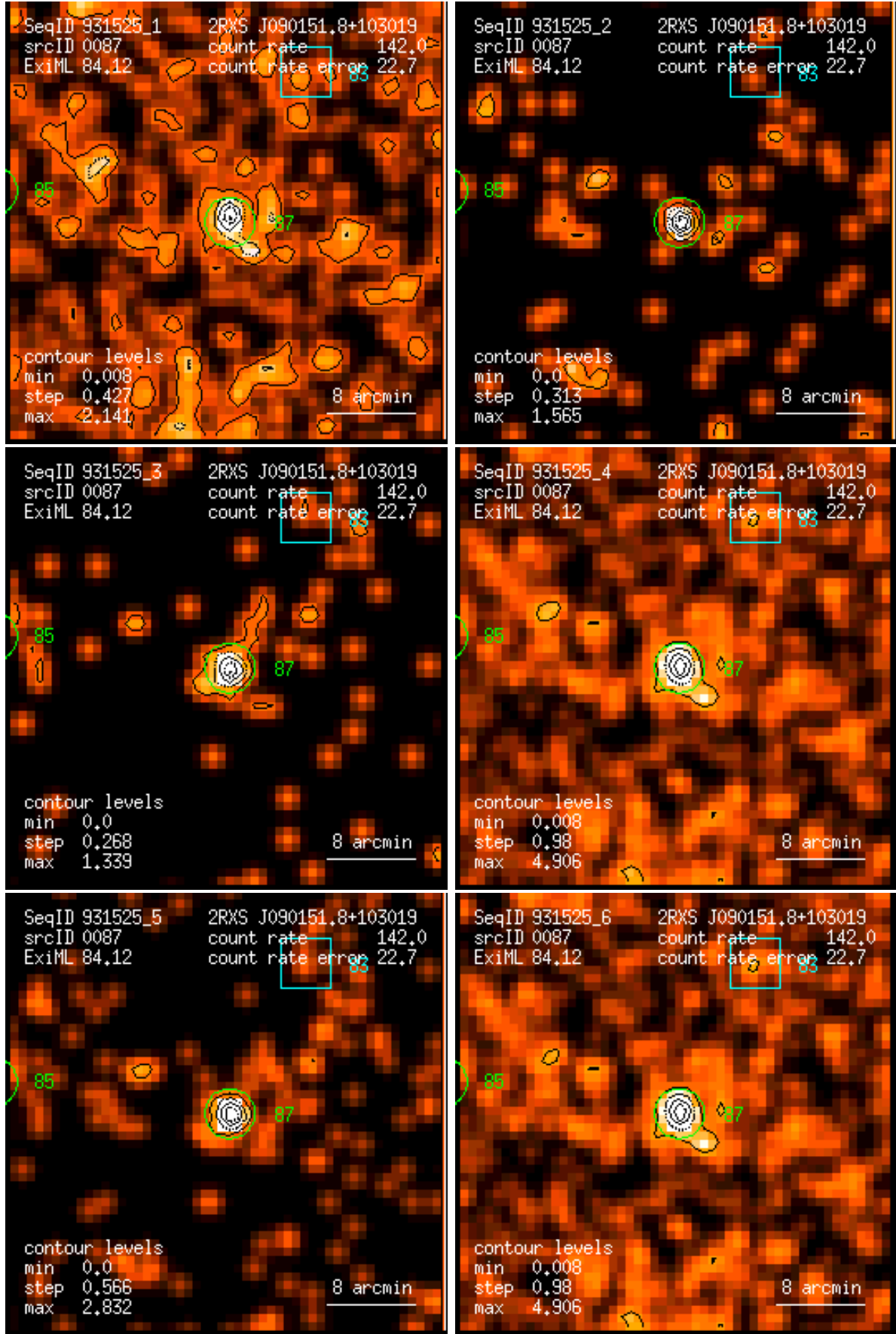
Figure 87: RASS 931525: detection 0087: band rate images, Gaussian filter: (1) PSPC channels 11 – 41, (2) 52 – 90, (3) 91 – 201, (4) 11 – 235, (5) 52 – 201, (6) 11 – 201. Broad band rates in counts/ks. Band rate contour levels in counts/ks/arcmin 2 .
