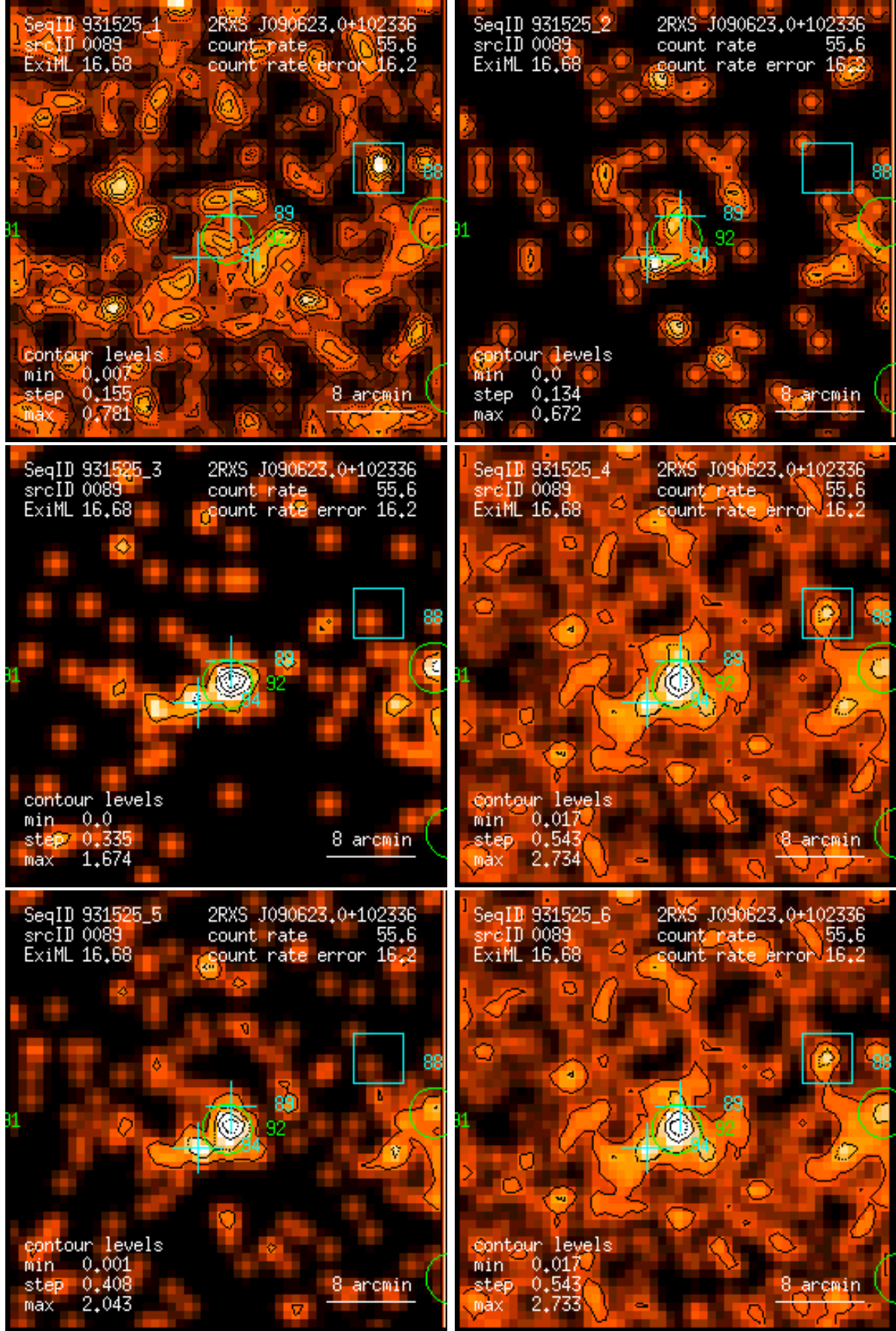
Figure 89: RASS 931525: detection 0089: band rate images, Gaussian filter: (1) PSPC channels 11 – 41, (2) 52 – 90, (3) 91 – 201, (4) 11 – 235, (5) 52 – 201, (6) 11 – 201. Broad band rates in counts/ks. Band rate contour levels in counts/ks/arcmin 2 .
