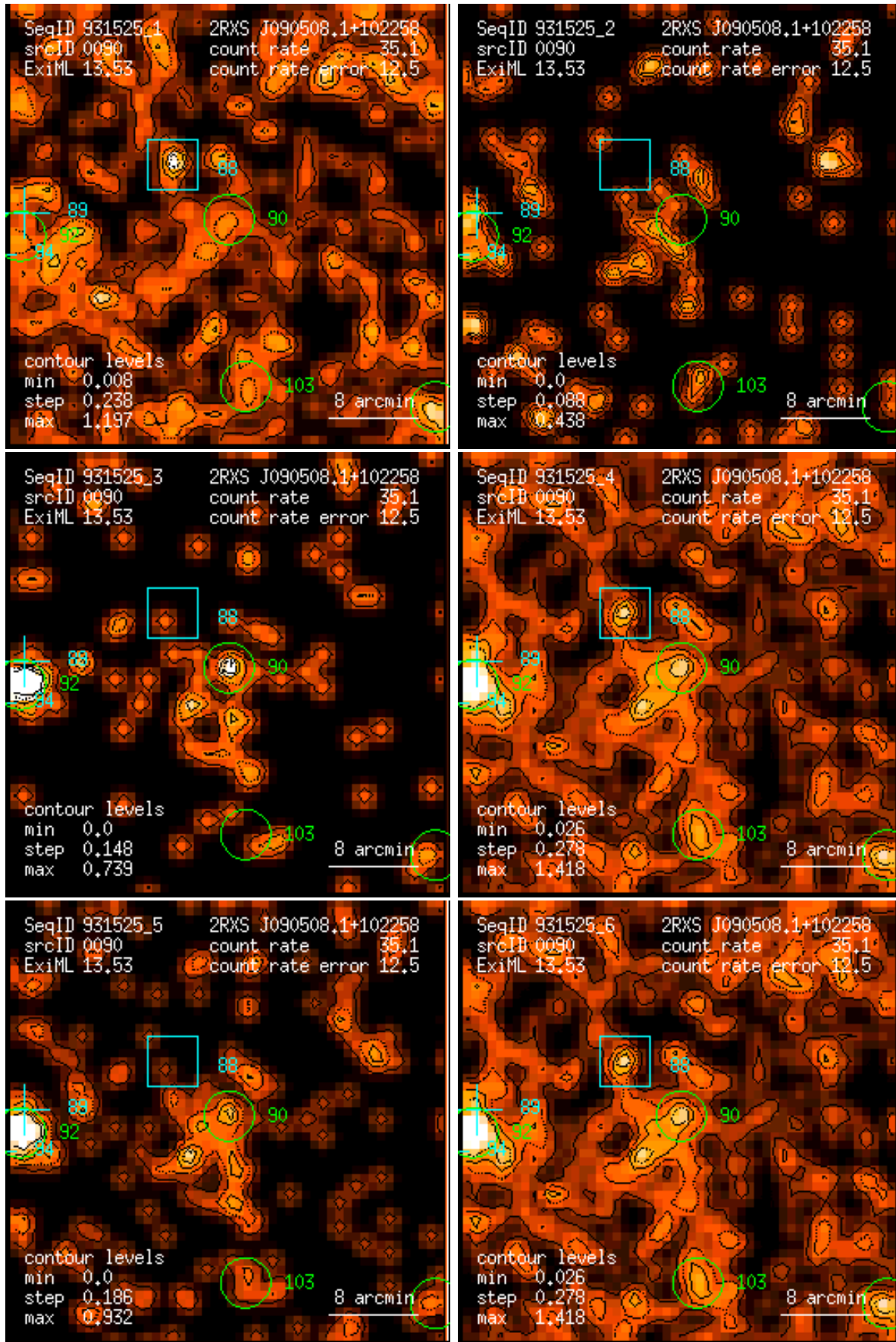
Figure 90: RASS 931525: detection 0090: band rate images, Gaussian filter: (1) PSPC channels 11 – 41, (2) 52 – 90, (3) 91 – 201, (4) 11 – 235, (5) 52 – 201, (6) 11 – 201. Broad band rates in counts/ks. Band rate contour levels in counts/ks/arcmin 2 .
