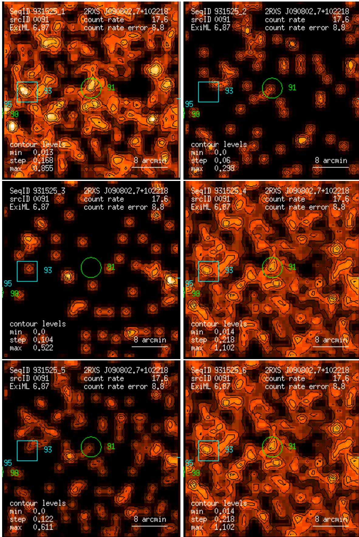
Figure 91: RASS 931525: detection 0091: band rate images, Gaussian filter: (1) PSPC channels 11 – 41, (2) 52 – 90, (3) 91 – 201, (4) 11 – 235, (5) 52 – 201, (6) 11 – 201. Broad band rates in counts/ks. Band rate contour levels in counts/ks/arcmin 2 .
