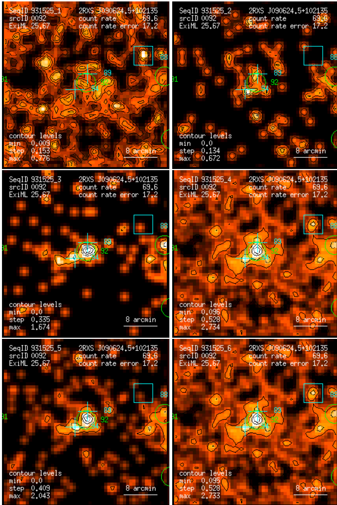
Figure 92: RASS 931525: detection 0092: band rate images, Gaussian filter: (1) PSPC channels 11 – 41, (2) 52 – 90, (3) 91 – 201, (4) 11 – 235, (5) 52 – 201, (6) 11 – 201. Broad band rates in counts/ks. Band rate contour levels in counts/ks/arcmin 2 .
