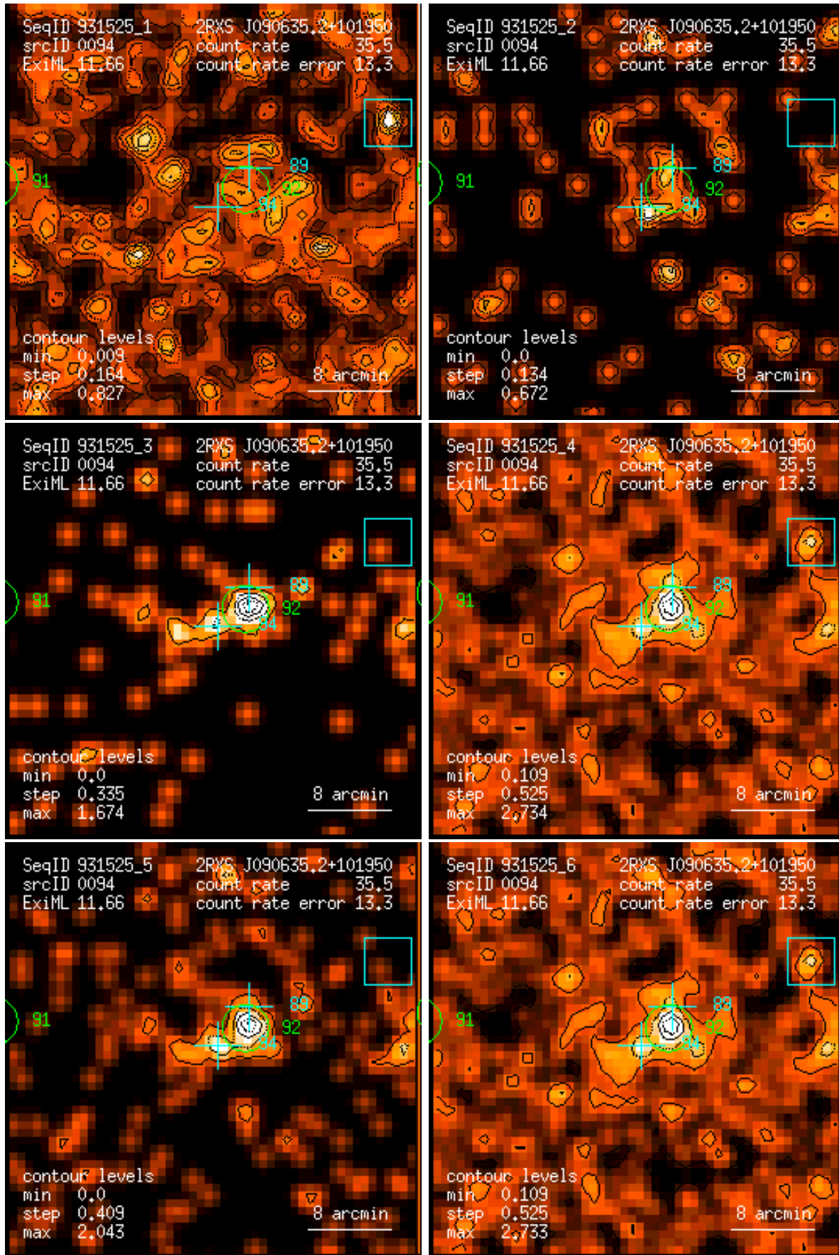
Figure 94: RASS 931525: detection 0094: band rate images, Gaussian filter: (1) PSPC channels 11 – 41, (2) 52 – 90, (3) 91 – 201, (4) 11 – 235, (5) 52 – 201, (6) 11 – 201. Broad band rates in counts/ks. Band rate contour levels in counts/ks/arcmin 2 .
