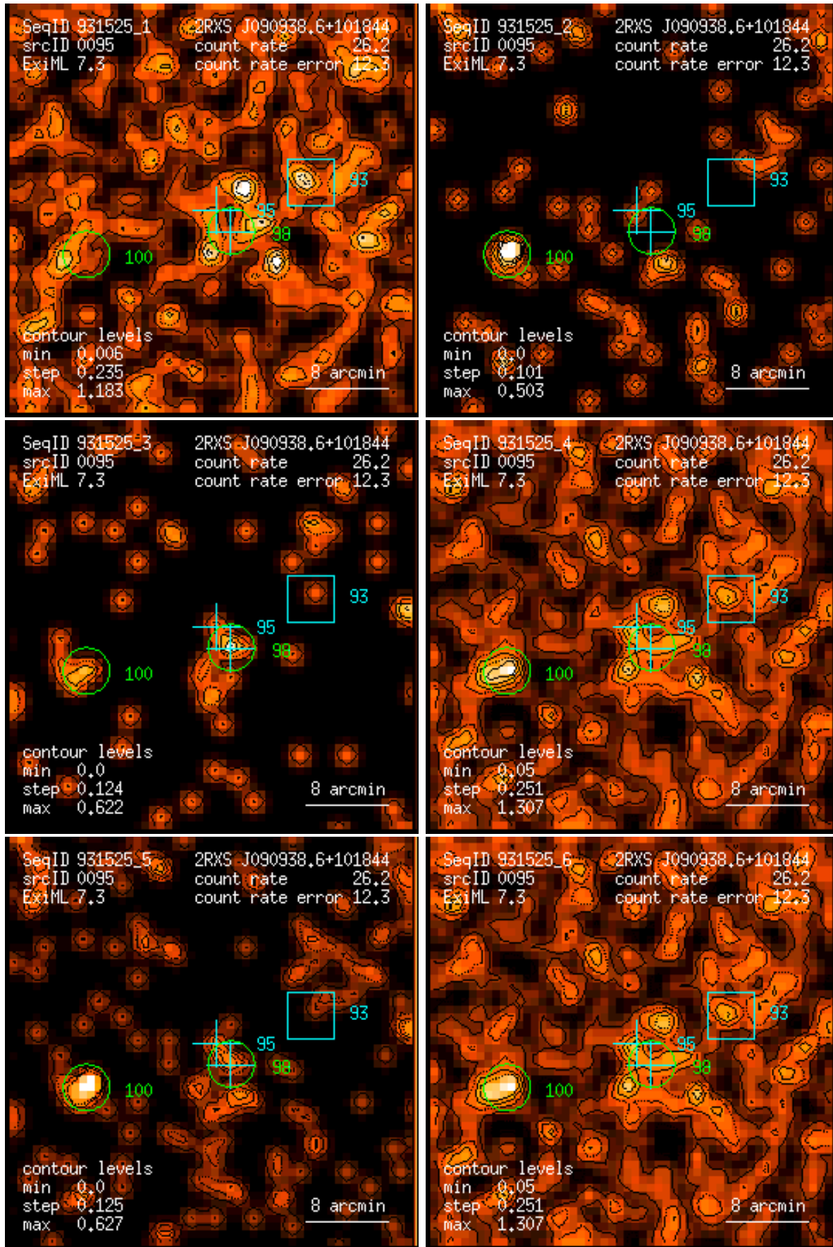
Figure 95: RASS 931525: detection 0095: band rate images, Gaussian filter: (1) PSPC channels 11 – 41, (2) 52 – 90, (3) 91 – 201, (4) 11 – 235, (5) 52 – 201, (6) 11 – 201. Broad band rates in counts/ks. Band rate contour levels in counts/ks/arcmin 2 .
