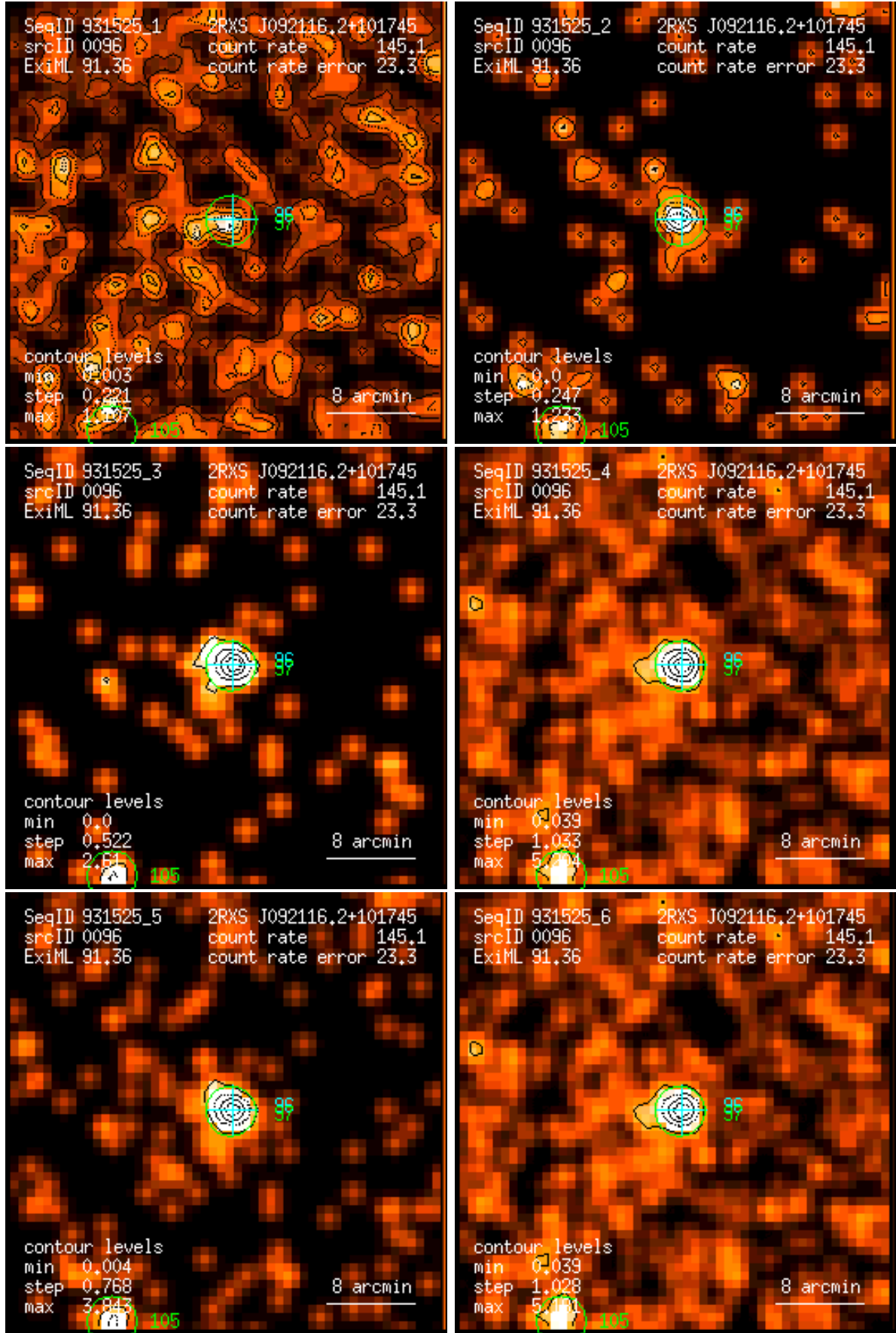
Figure 96: RASS 931525: detection 0096: band rate images, Gaussian filter: (1) PSPC channels 11 – 41, (2) 52 – 90, (3) 91 – 201, (4) 11 – 235, (5) 52 – 201, (6) 11 – 201. Broad band rates in counts/ks. Band rate contour levels in counts/ks/arcmin 2 .
