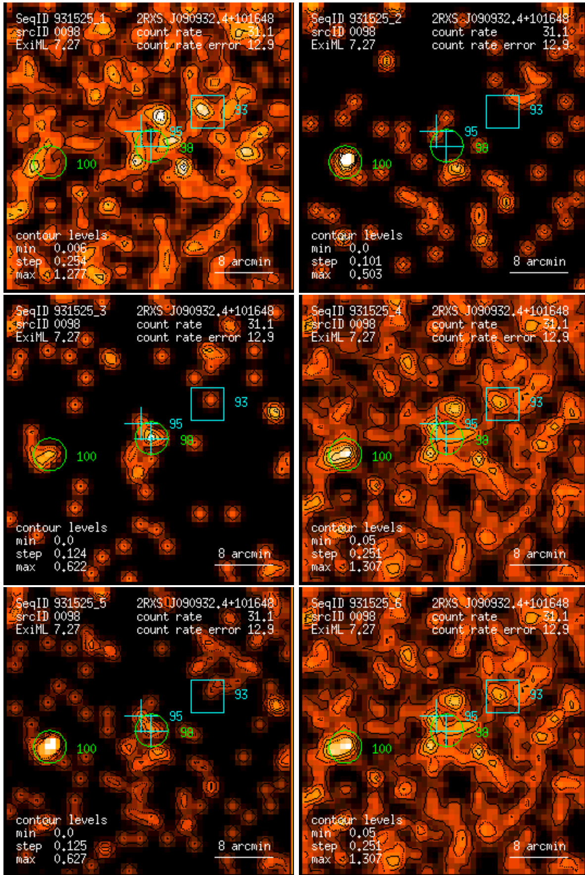
Figure 98: RASS 931525: detection 0098: band rate images, Gaussian filter: (1) PSPC channels 11 – 41, (2) 52 – 90, (3) 91 – 201, (4) 11 – 235, (5) 52 – 201, (6) 11 – 201. Broad band rates in counts/ks. Band rate contour levels in counts/ks/arcmin 2 .
