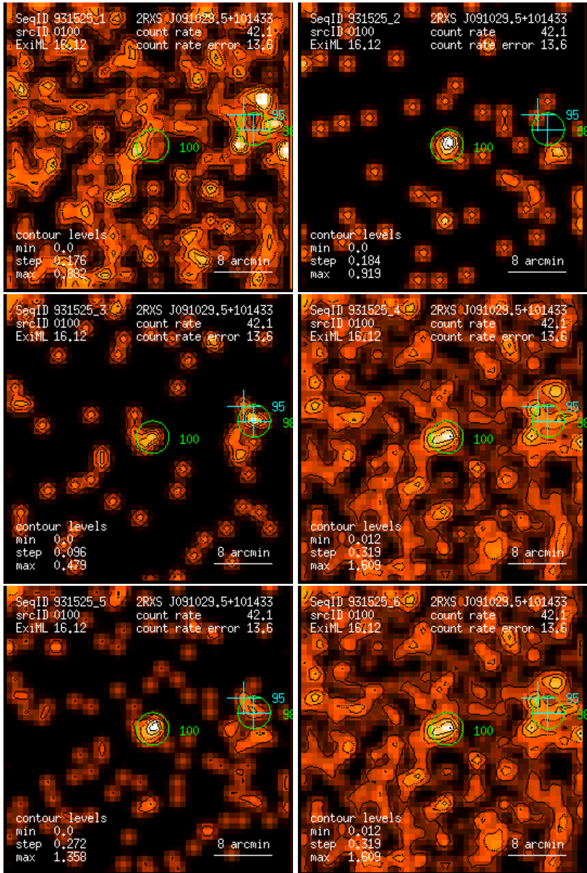
Figure 100: RASS 931525: detection 0100: band rate images, Gaussian filter: (1) PSPC channels 11 – 41, (2) 52 – 90, (3) 91 – 201, (4) 11 – 235, (5) 52 – 201, (6) 11 – 201. Broad band rates in counts/ks. Band rate contour levels in counts/ks/arcmin 2 .
