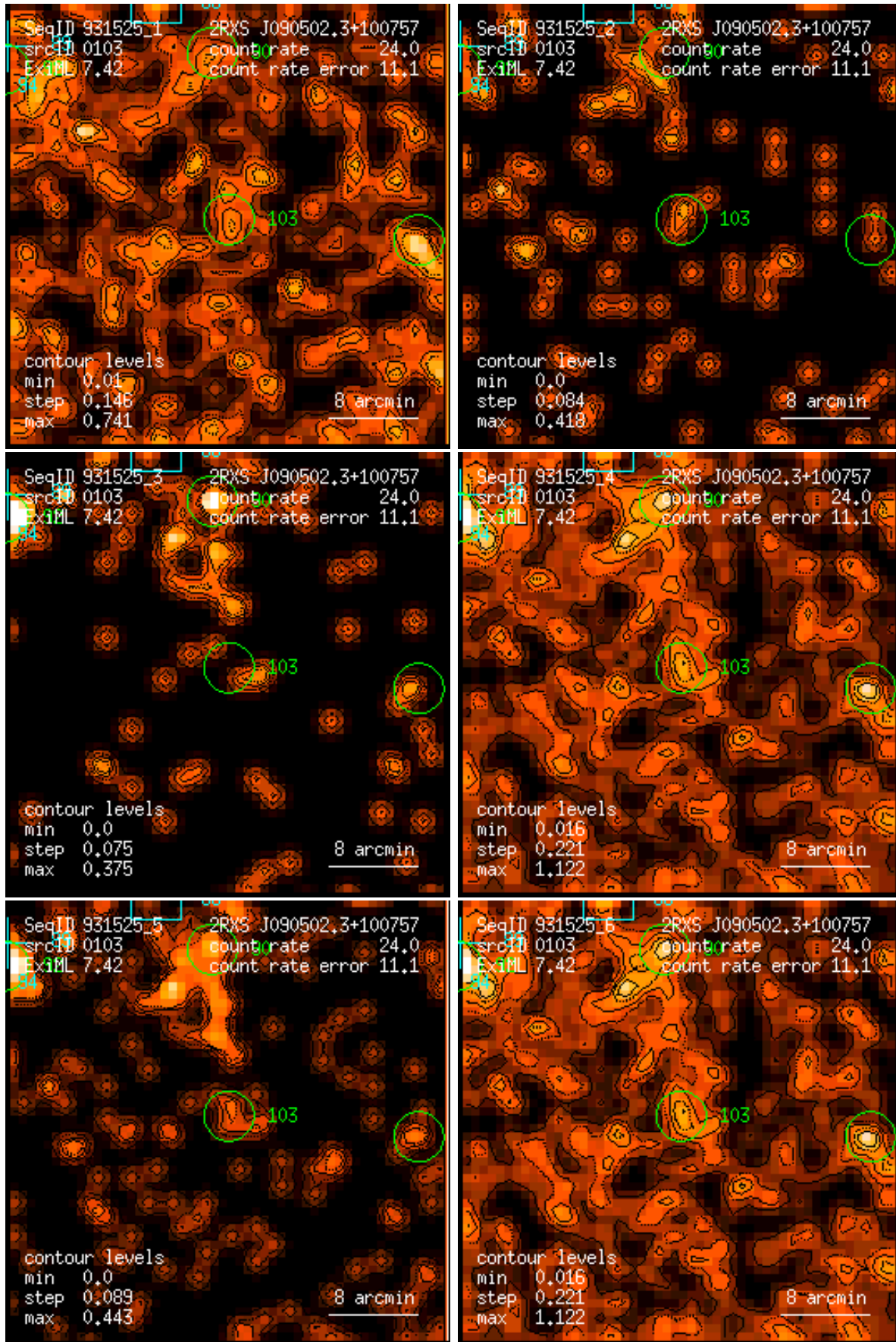
Figure 103: RASS 931525: detection 0103: band rate images, Gaussian filter: (1) PSPC channels 11 – 41, (2) 52 – 90, (3) 91 – 201, (4) 11 – 235, (5) 52 – 201, (6) 11 – 201. Broad band rates in counts/ks. Band rate contour levels in counts/ks/arcmin 2 .
