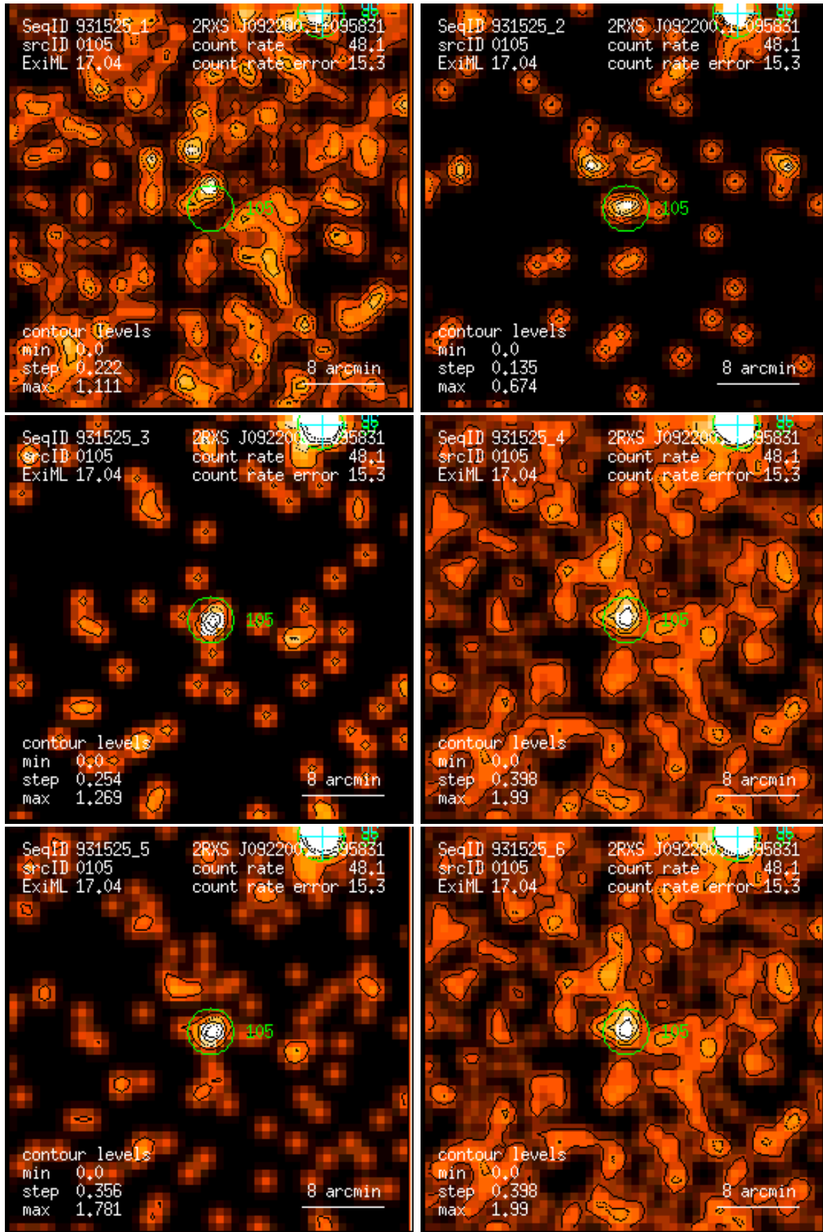
Figure 105: RASS 931525: detection 0105: band rate images, Gaussian filter: (1) PSPC channels 11 – 41, (2) 52 – 90, (3) 91 – 201, (4) 11 – 235, (5) 52 – 201, (6) 11 – 201. Broad band rates in counts/ks. Band rate contour levels in counts/ks/arcmin 2 .
