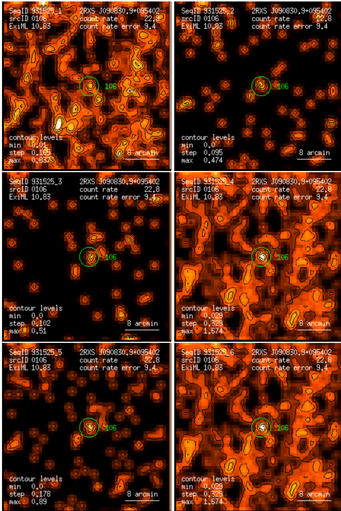
Figure 106: RASS 931525: detection 0106: band rate images, Gaussian filter: (1) PSPC channels 11 – 41, (2) 52 – 90, (3) 91 – 201, (4) 11 – 235, (5) 52 – 201, (6) 11 – 201. Broad band rates in counts/ks. Band rate contour levels in counts/ks/arcmin 2 .
