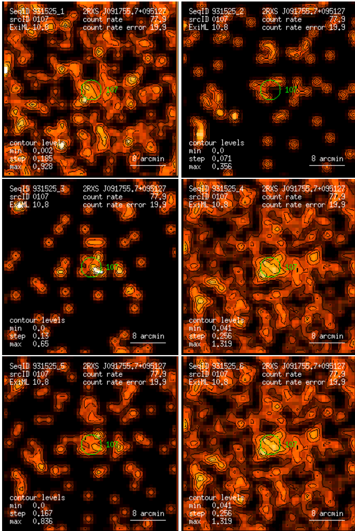
Figure 107: RASS 931525: detection 0107: band rate images, Gaussian filter: (1) PSPC channels 11 – 41, (2) 52 – 90, (3) 91 – 201, (4) 11 – 235, (5) 52 – 201, (6) 11 – 201. Broad band rates in counts/ks. Band rate contour levels in counts/ks/arcmin 2 .
