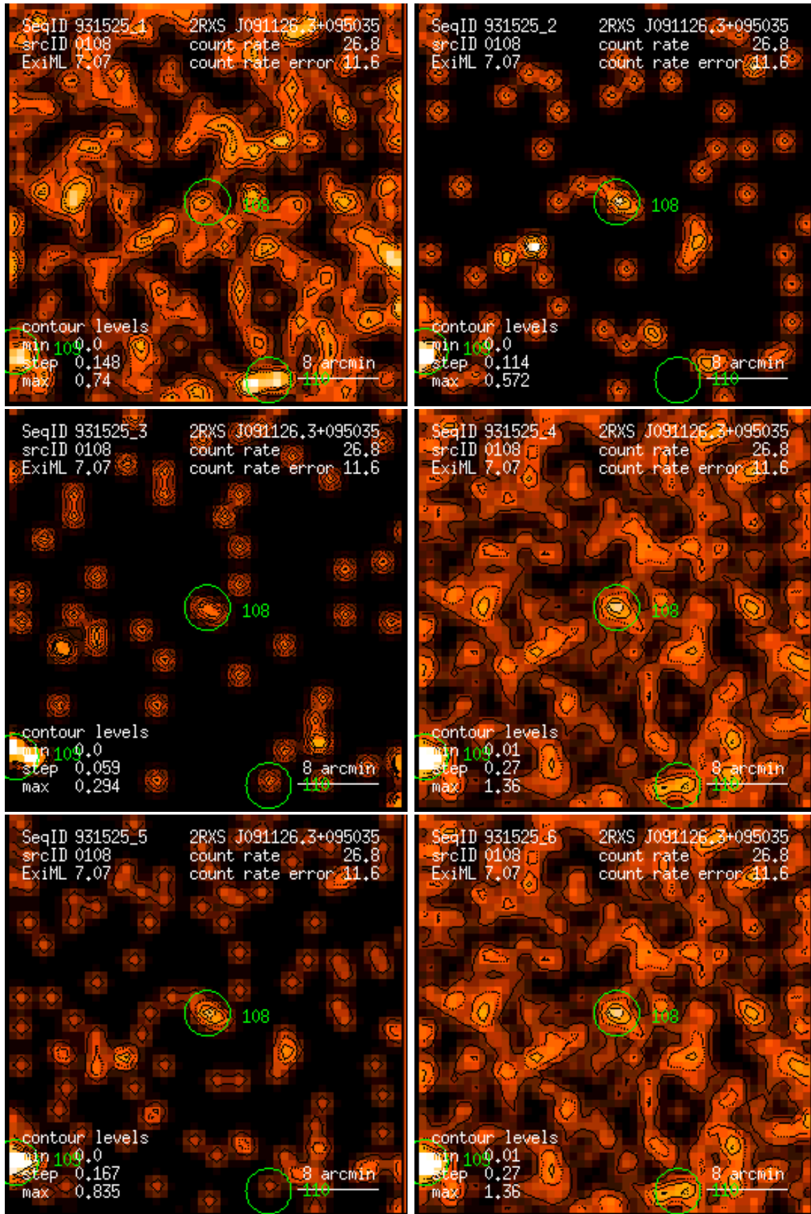
Figure 108: RASS 931525: detection 0108: band rate images, Gaussian filter: (1) PSPC channels 11 – 41, (2) 52 – 90, (3) 91 – 201, (4) 11 – 235, (5) 52 – 201, (6) 11 – 201. Broad band rates in counts/ks. Band rate contour levels in counts/ks/arcmin 2 .
