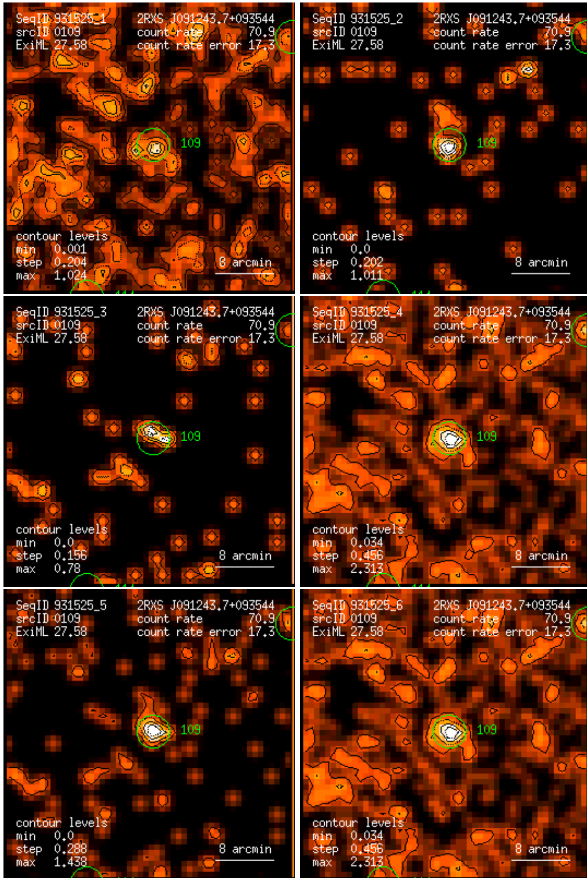
Figure 109: RASS 931525: detection 0109: band rate images, Gaussian filter: (1) PSPC channels 11 – 41, (2) 52 – 90, (3) 91 – 201, (4) 11 – 235, (5) 52 – 201, (6) 11 – 201. Broad band rates in counts/ks. Band rate contour levels in counts/ks/arcmin 2 .
