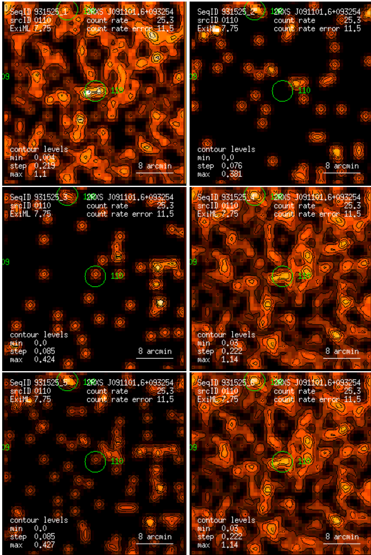
Figure 110: RASS 931525: detection 0110: band rate images, Gaussian filter: (1) PSPC channels 11 – 41, (2) 52 – 90, (3) 91 – 201, (4) 11 – 235, (5) 52 – 201, (6) 11 – 201. Broad band rates in counts/ks. Band rate contour levels in counts/ks/arcmin 2 .
