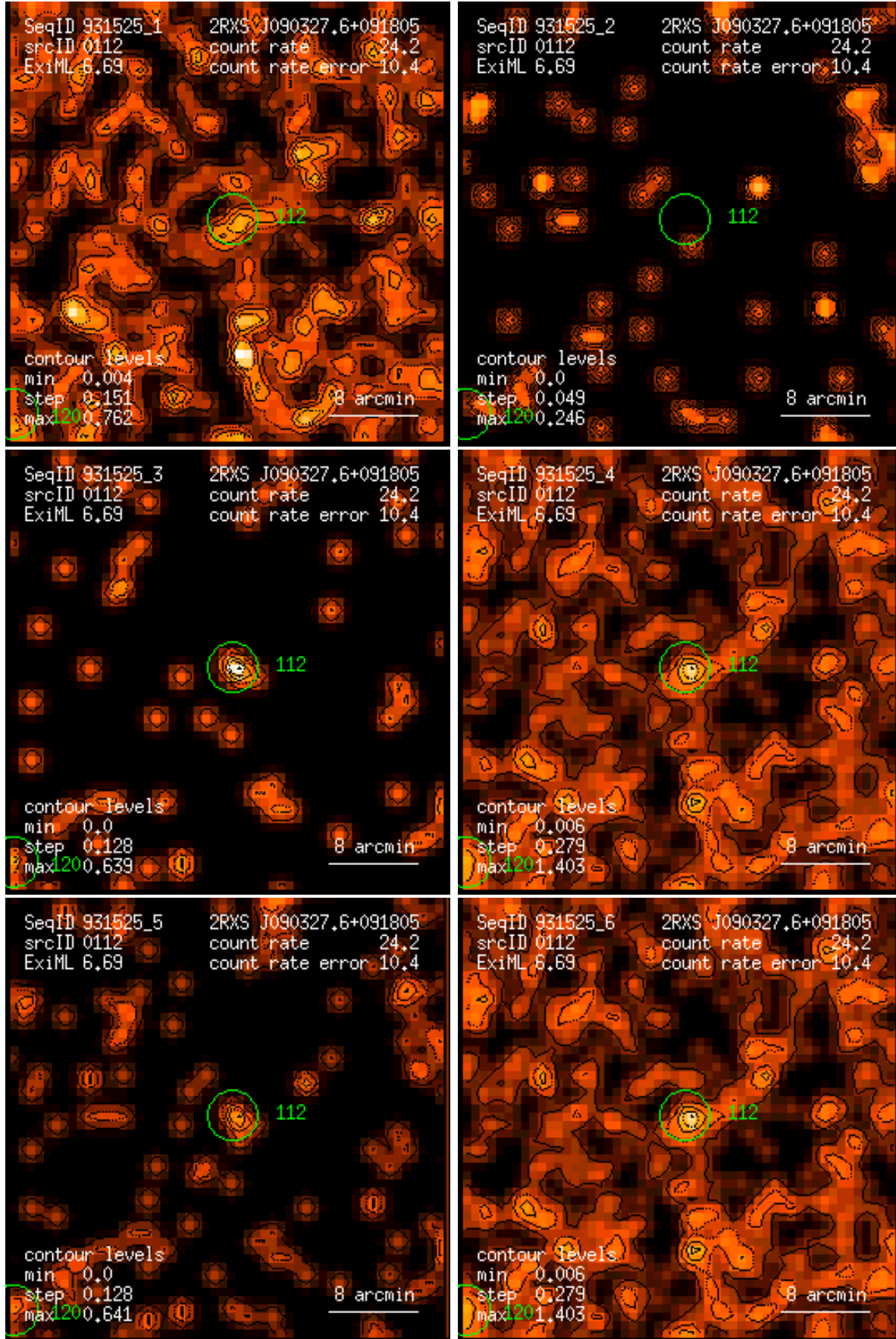
Figure 112: RASS 931525: detection 0112: band rate images, Gaussian filter: (1) PSPC channels 11 – 41, (2) 52 – 90, (3) 91 – 201, (4) 11 – 235, (5) 52 – 201, (6) 11 – 201. Broad band rates in counts/ks. Band rate contour levels in counts/ks/arcmin 2 .
