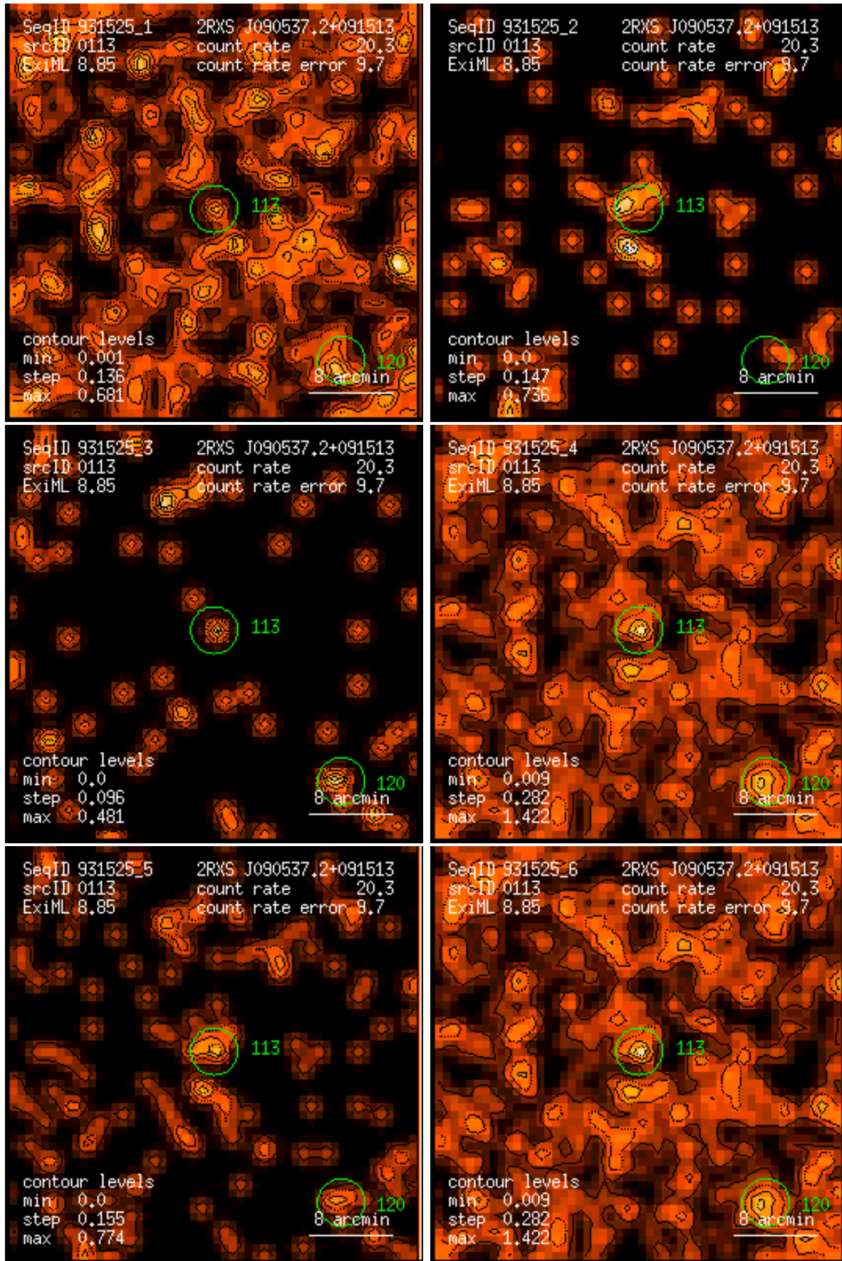
Figure 113: RASS 931525: detection 0113: band rate images, Gaussian filter: (1) PSPC channels 11 – 41, (2) 52 – 90, (3) 91 – 201, (4) 11 – 235, (5) 52 – 201, (6) 11 – 201. Broad band rates in counts/ks. Band rate contour levels in counts/ks/arcmin 2 .
