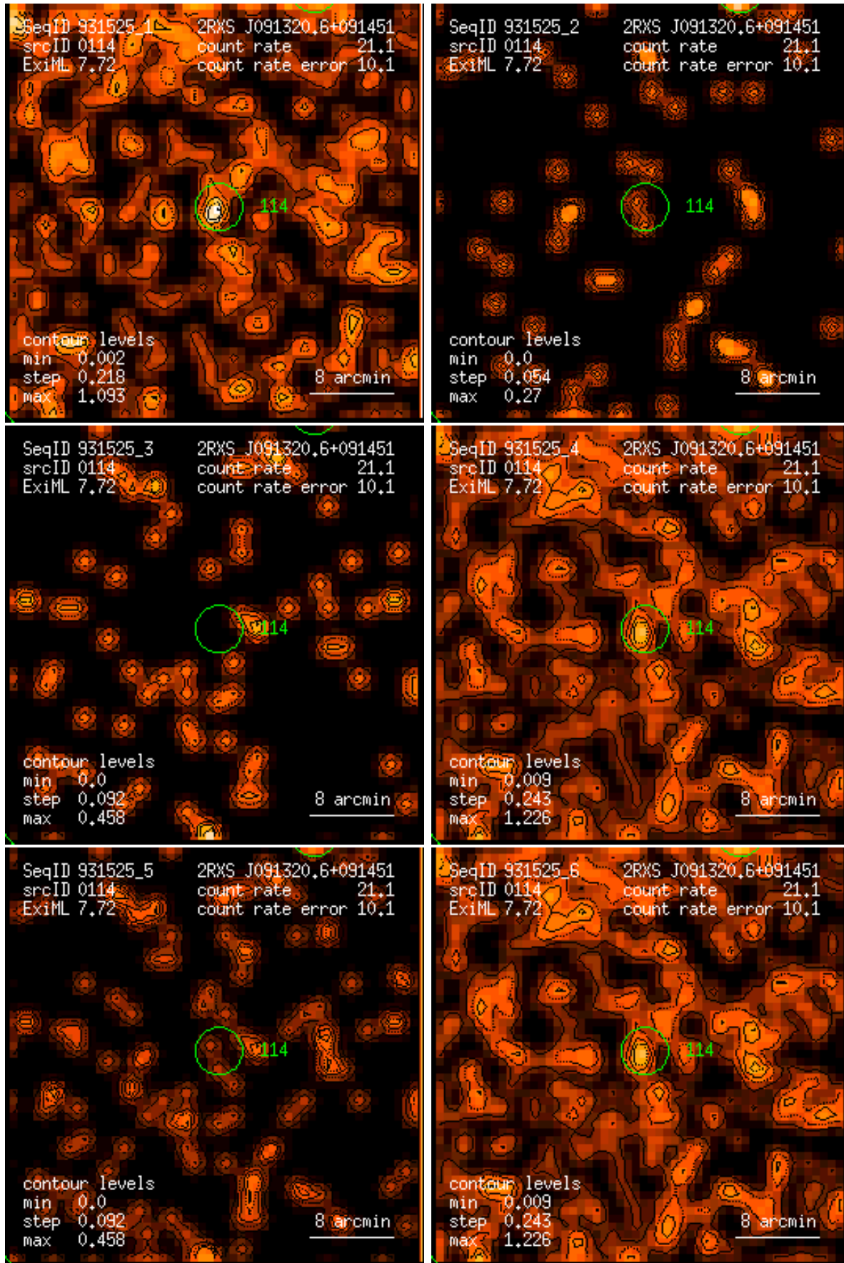
Figure 114: RASS 931525: detection 0114: band rate images, Gaussian filter: (1) PSPC channels 11 – 41, (2) 52 – 90, (3) 91 – 201, (4) 11 – 235, (5) 52 – 201, (6) 11 – 201. Broad band rates in counts/ks. Band rate contour levels in counts/ks/arcmin 2 .
