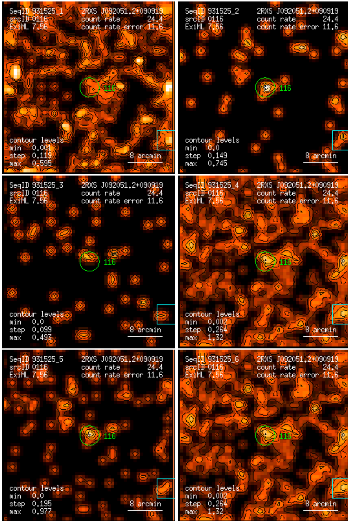
Figure 116: RASS 931525: detection 0116: band rate images, Gaussian filter: (1) PSPC channels 11 – 41, (2) 52 – 90, (3) 91 – 201, (4) 11 – 235, (5) 52 – 201, (6) 11 – 201. Broad band rates in counts/ks. Band rate contour levels in counts/ks/arcmin 2 .
