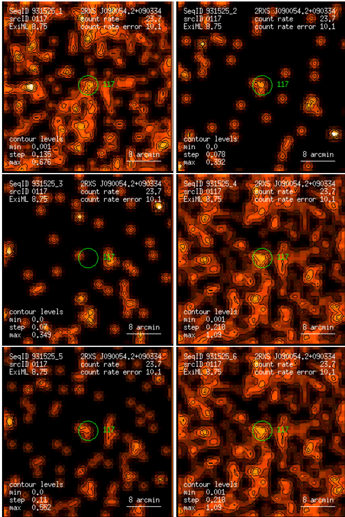
Figure 117: RASS 931525: detection 0117: band rate images, Gaussian filter: (1) PSPC channels 11 – 41, (2) 52 – 90, (3) 91 – 201, (4) 11 – 235, (5) 52 – 201, (6) 11 – 201. Broad band rates in counts/ks. Band rate contour levels in counts/ks/arcmin 2 .
