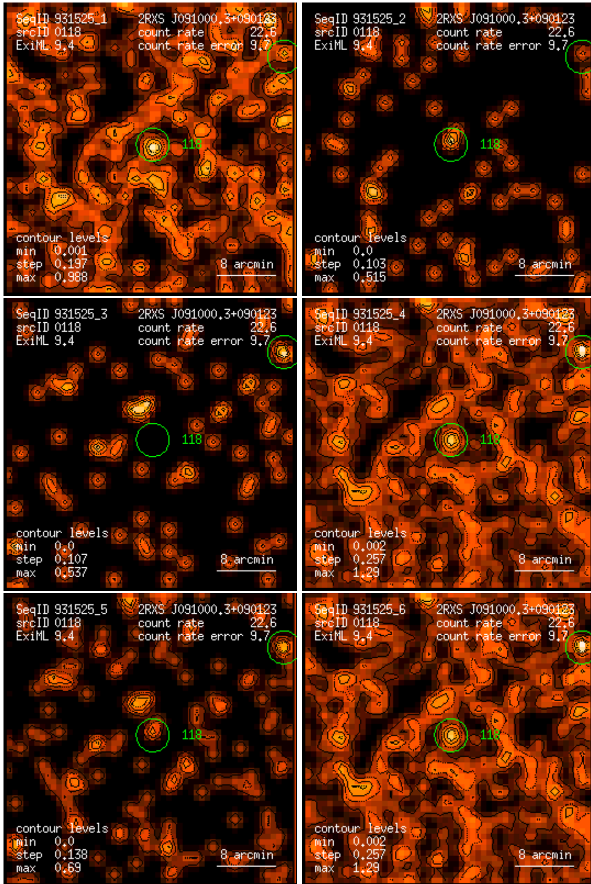
Figure 118: RASS 931525: detection 0118: band rate images, Gaussian filter: (1) PSPC channels 11 – 41, (2) 52 – 90, (3) 91 – 201, (4) 11 – 235, (5) 52 – 201, (6) 11 – 201. Broad band rates in counts/ks. Band rate contour levels in counts/ks/arcmin 2 .
