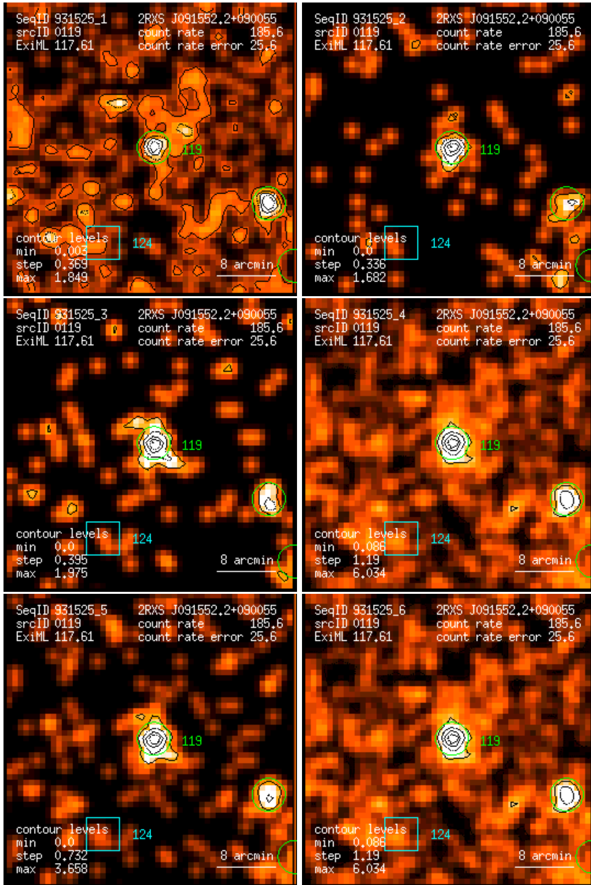
Figure 119: RASS 931525: detection 0119: band rate images, Gaussian filter: (1) PSPC channels 11 – 41, (2) 52 – 90, (3) 91 – 201, (4) 11 – 235, (5) 52 – 201, (6) 11 – 201. Broad band rates in counts/ks. Band rate contour levels in counts/ks/arcmin 2 .
