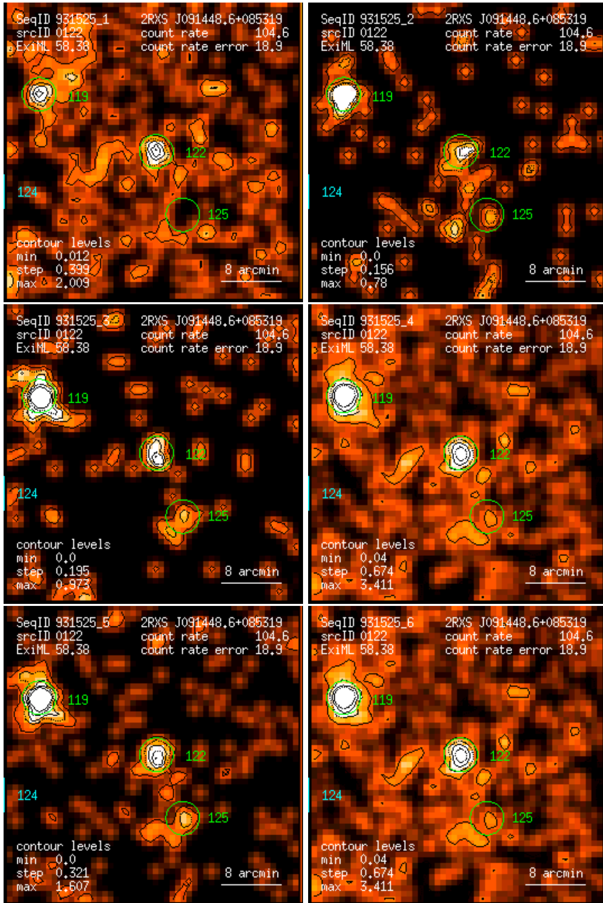
Figure 122: RASS 931525: detection 0122: band rate images, Gaussian filter: (1) PSPC channels 11 – 41, (2) 52 – 90, (3) 91 – 201, (4) 11 – 235, (5) 52 – 201, (6) 11 – 201. Broad band rates in counts/ks. Band rate contour levels in counts/ks/arcmin 2 .
