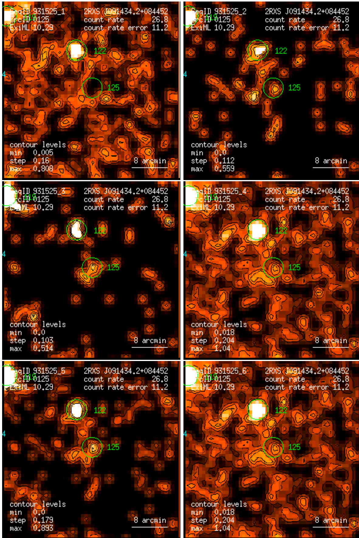
Figure 125: RASS 931525: detection 0125: band rate images, Gaussian filter: (1) PSPC channels 11 – 41, (2) 52 – 90, (3) 91 – 201, (4) 11 – 235, (5) 52 – 201, (6) 11 – 201. Broad band rates in counts/ks. Band rate contour levels in counts/ks/arcmin 2 .
