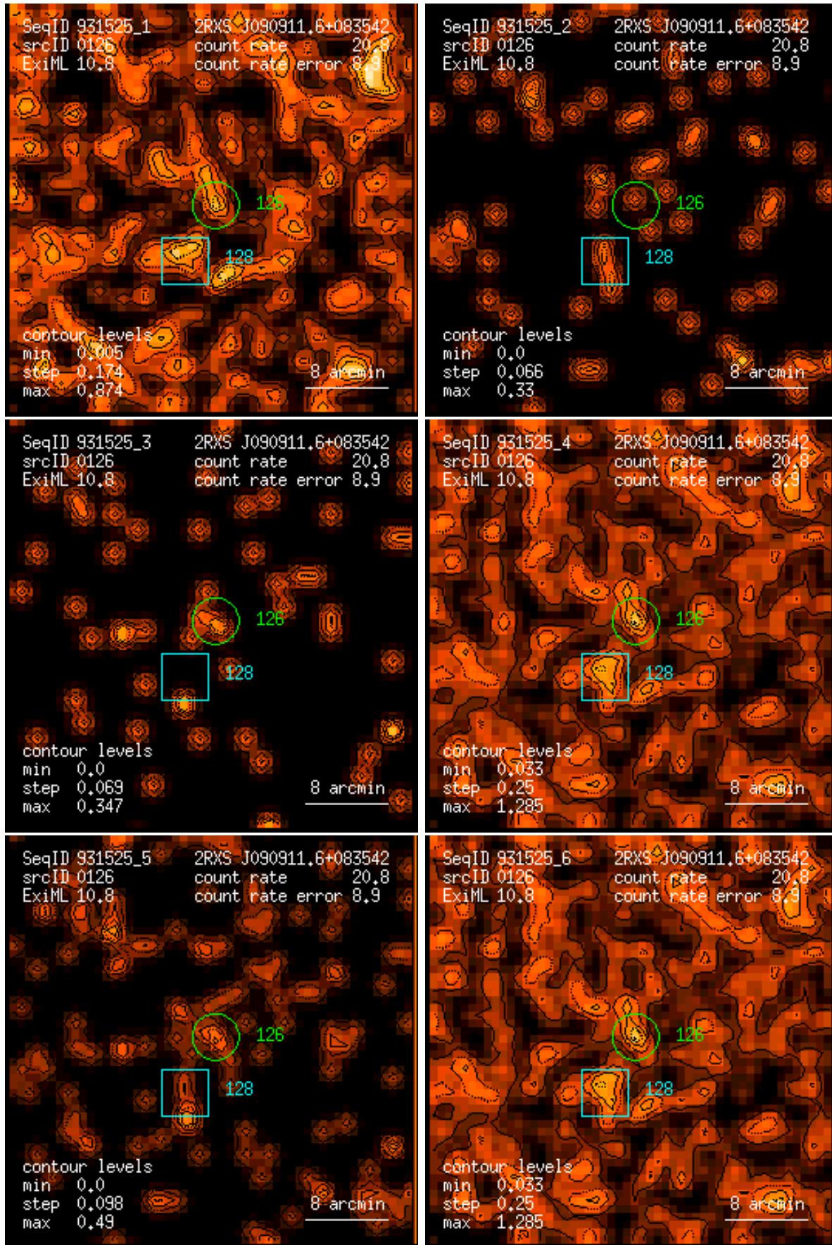
Figure 126: RASS 931525: detection 0126: band rate images, Gaussian filter: (1) PSPC channels 11 – 41, (2) 52 – 90, (3) 91 – 201, (4) 11 – 235, (5) 52 – 201, (6) 11 – 201. Broad band rates in counts/ks. Band rate contour levels in counts/ks/arcmin 2 .
