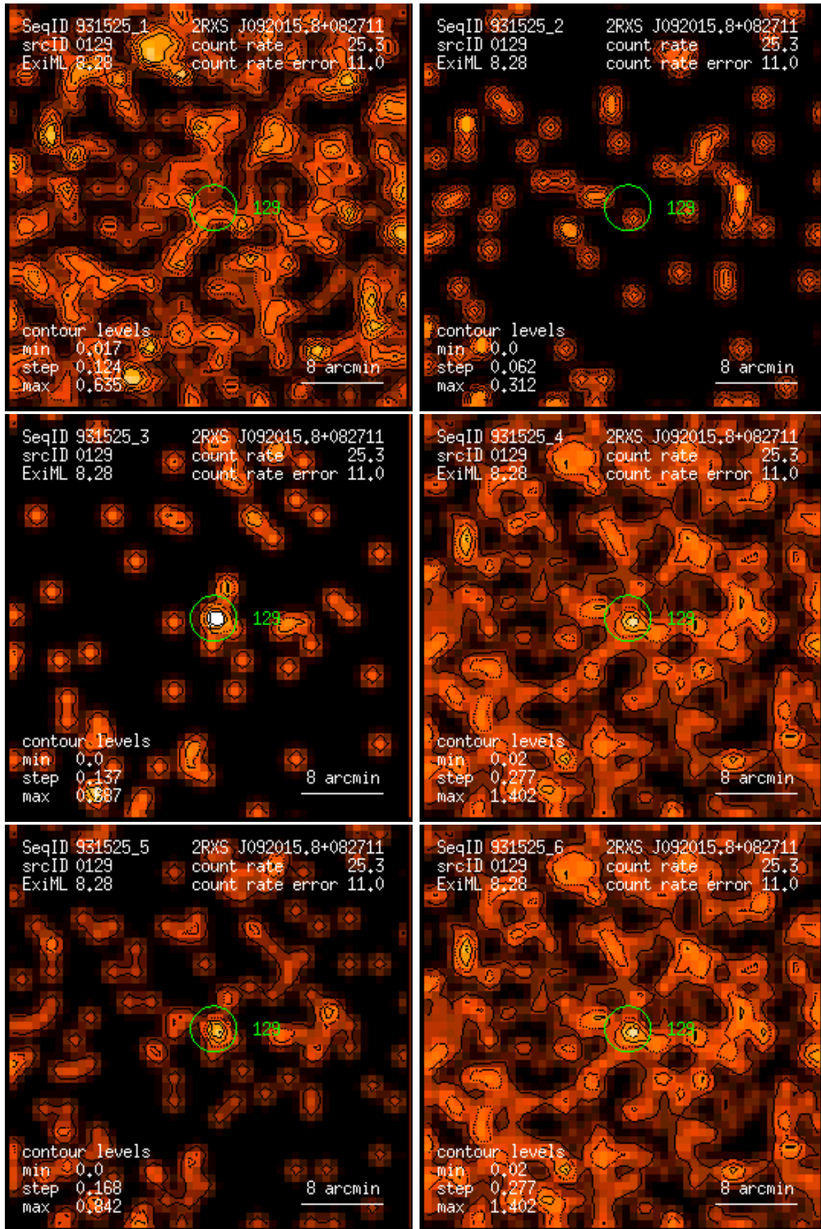
Figure 129: RASS 931525: detection 0129: band rate images, Gaussian filter: (1) PSPC channels 11 – 41, (2) 52 – 90, (3) 91 – 201, (4) 11 – 235, (5) 52 – 201, (6) 11 – 201. Broad band rates in counts/ks. Band rate contour levels in counts/ks/arcmin 2 .
