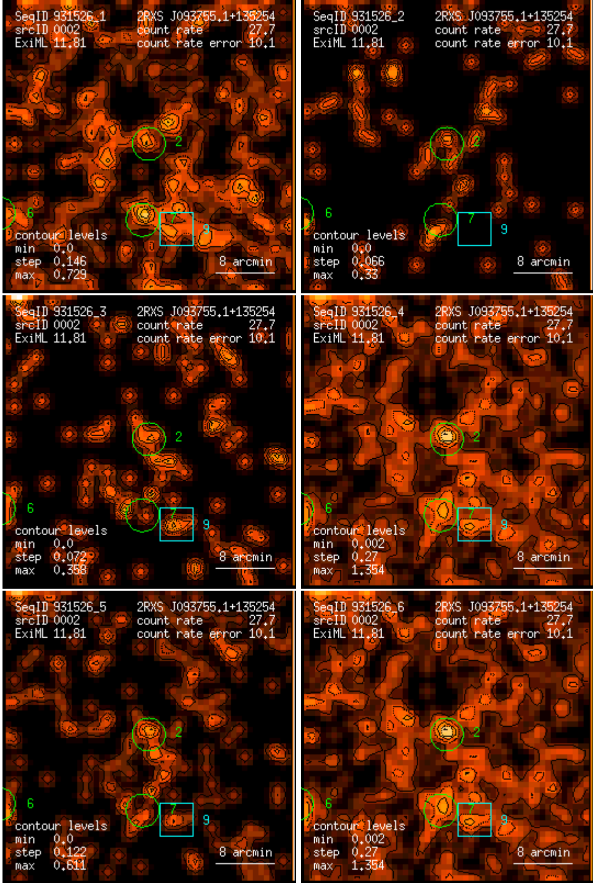
Figure 2: RASS 931526: detection 0002: band rate images, Gaussian filter: (1) PSPC channels 11 – 41, (2) 52 – 90, (3) 91 – 201, (4) 11 – 235, (5) 52 – 201, (6) 11 – 201. Broad band rates in counts/ks. Band rate contour levels in counts/ks/arcmin 2 .
