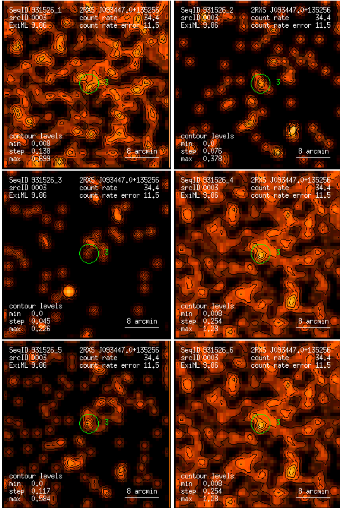
Figure 3: RASS 931526: detection 0003: band rate images, Gaussian filter: (1) PSPC channels 11 – 41, (2) 52 – 90, (3) 91 – 201, (4) 11 – 235, (5) 52 – 201, (6) 11 – 201. Broad band rates in counts/ks. Band rate contour levels in counts/ks/arcmin 2 .
