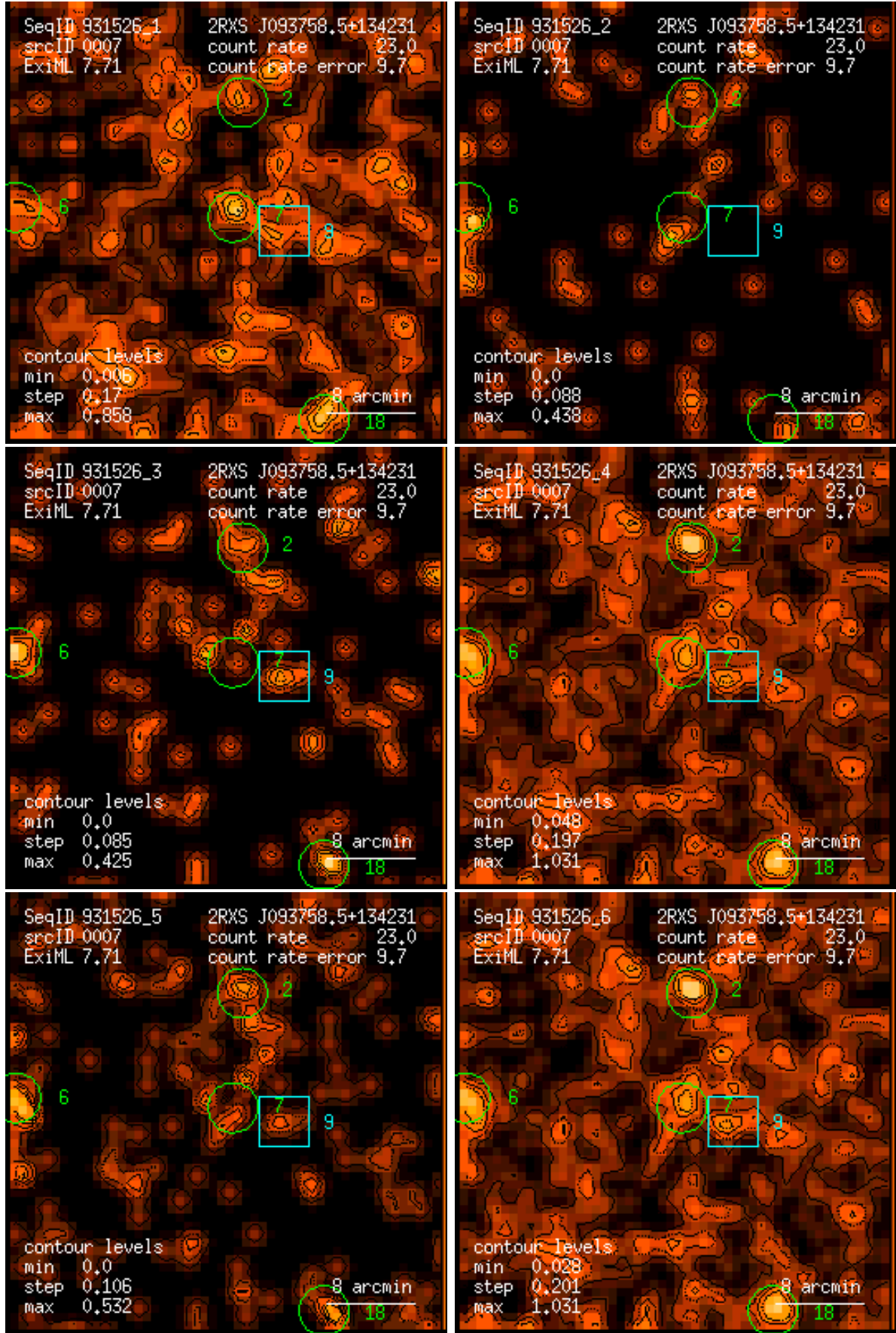
Figure 7: RASS 931526: detection 0007: band rate images, Gaussian filter: (1) PSPC channels 11 – 41, (2) 52 – 90, (3) 91 – 201, (4) 11 – 235, (5) 52 – 201, (6) 11 – 201. Broad band rates in counts/ks. Band rate contour levels in counts/ks/arcmin 2 .
