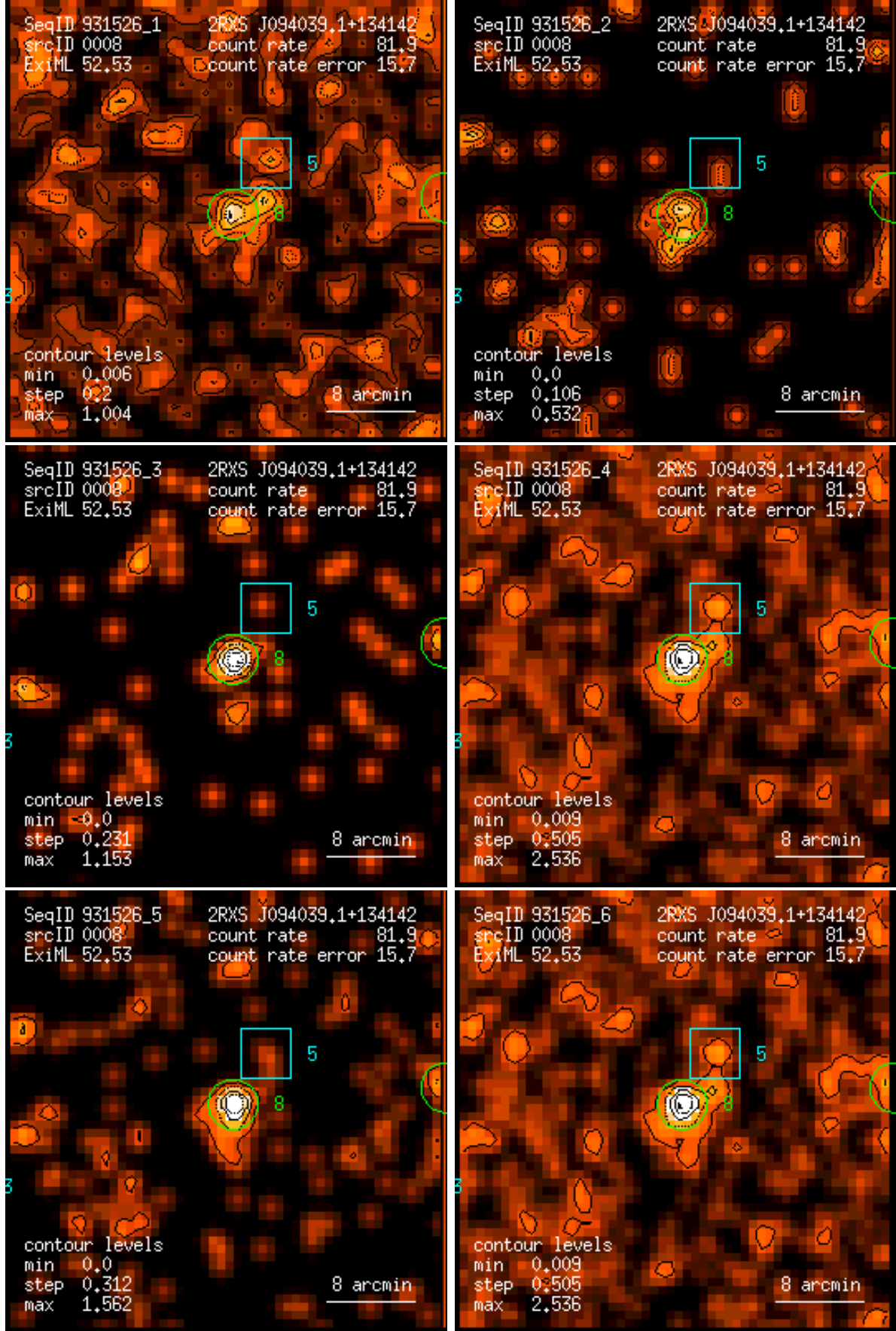
Figure 8: RASS 931526: detection 0008: band rate images, Gaussian filter: (1) PSPC channels 11 – 41, (2) 52 – 90, (3) 91 – 201, (4) 11 – 235, (5) 52 – 201, (6) 11 – 201. Broad band rates in counts/ks. Band rate contour levels in counts/ks/arcmin 2 .
